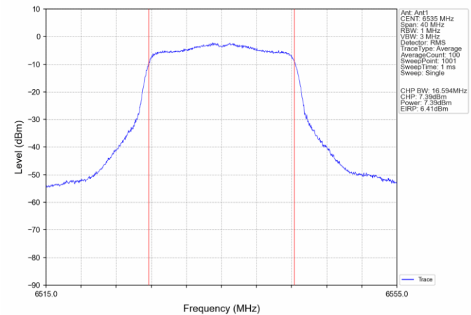
802.11a_LCH_6535MHz_Ant1_NTV
