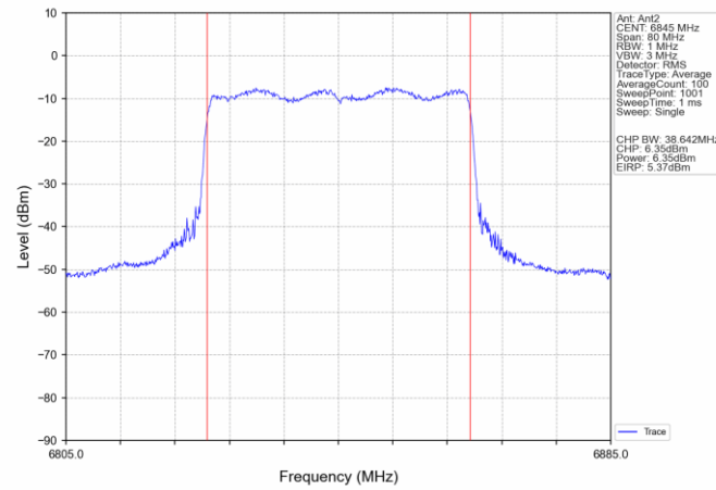
802.11ax(HEW40) HCH_6845MHz_SU_ / Ant2_NTNV
