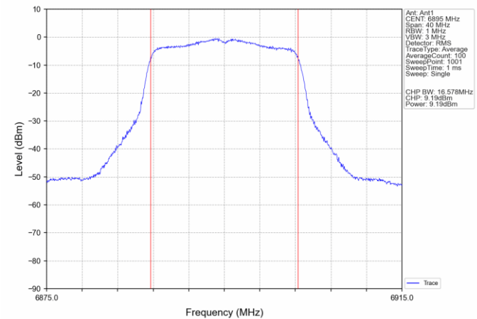
802.11a_LCH_6895MHz_Ant1_NTV
