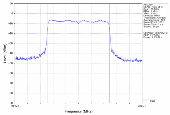
802.11ax(HEW40)_MCH_7005MHz_SU_ / Ant1_NTNV
