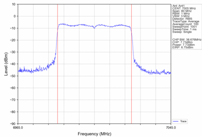
802.11ax(HEW40)_MCH_7005MHz_SU_ / Ant1_NTNV
