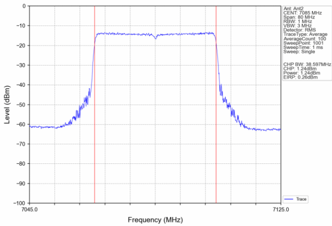
802.11ax(HEW40) HCH_7085MHz_SU_ / Ant2_NTNV
