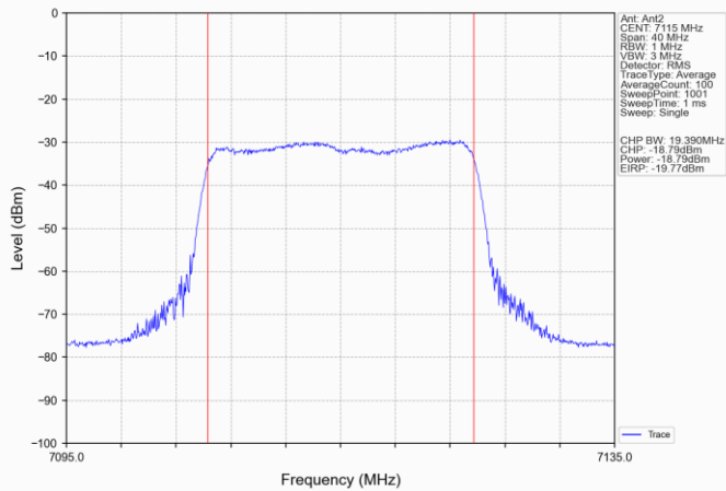
802.11ax(HEW20) HCH_7115MHz_SU_ / Ant2_NTNV
