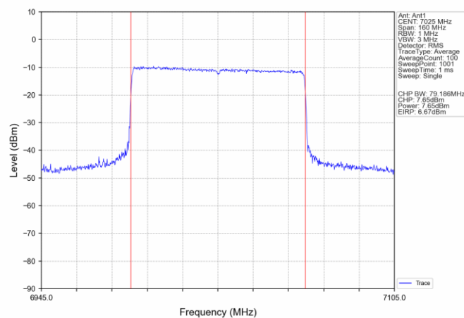
802.11ax(HEW80)_HCH_7025MHz_SU_ / Ant1_NTNV
