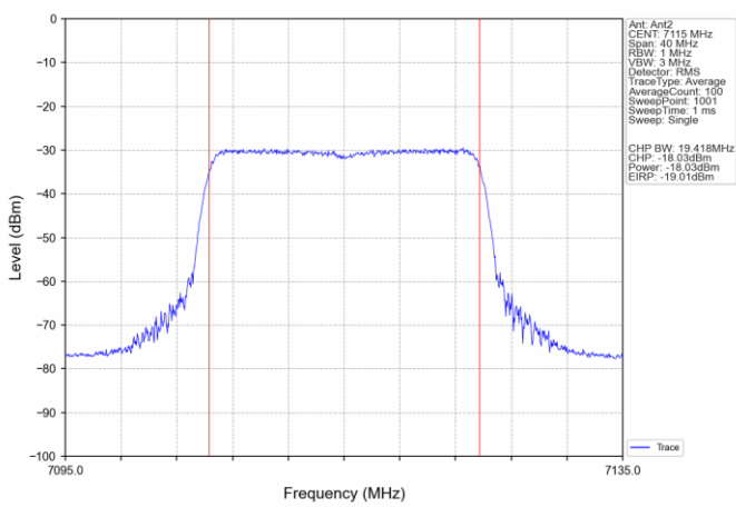
802.11ax(HEW20) HCH_7115MHz_SU_ / Ant2_NTNV
