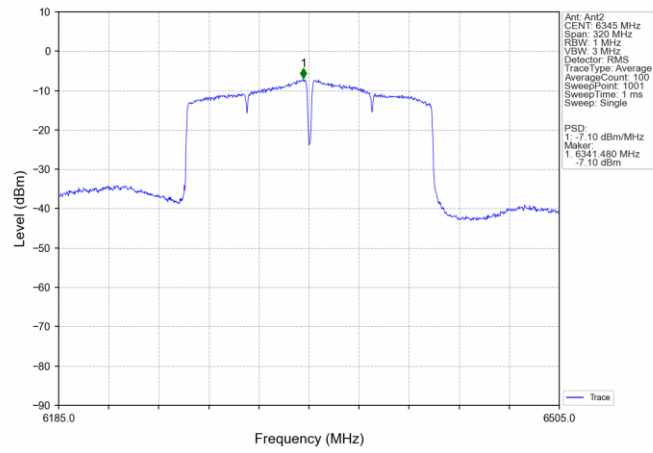
802.11ac(VHT160) HCH_6345MHz_Ant2_NTNV
