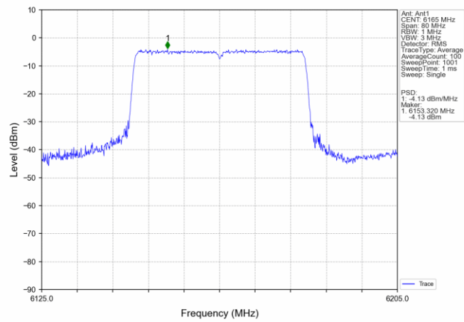
802.11ax(HEW40)_MCH_6165MHz_SU_ / Ant1_NTNV
