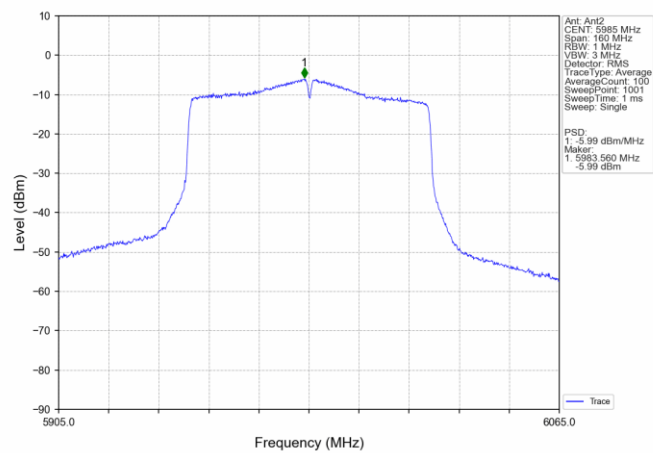
802.11ac(VHT80)_LCH_5985MHz_MIMO_NTNV
