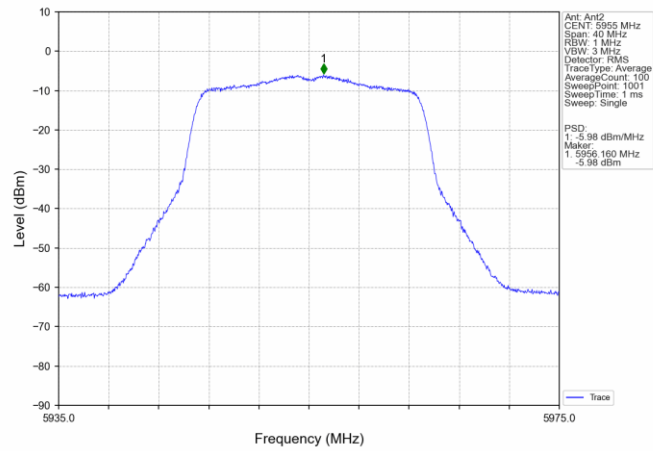
802.11ac(VHT20)_LCH_5955MHz_MIMO_NTNV
