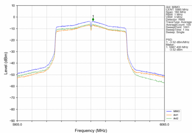
802.11ac(VHT80)_LCH_5985MHz_MIMO_NTNV
