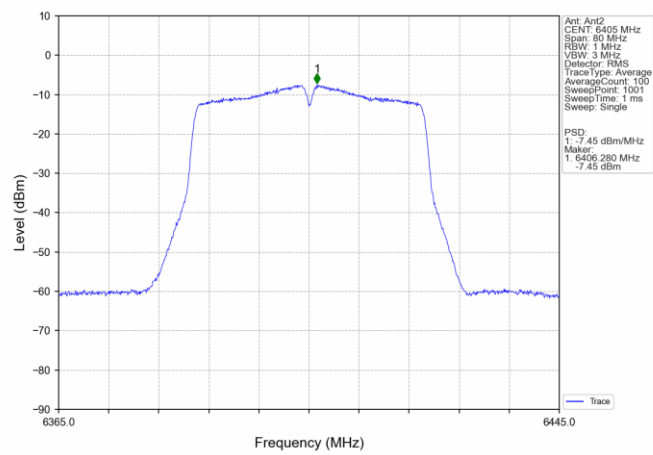
802.11ac(VHT40) HCH_6405MHz_MIMO_NTNV
