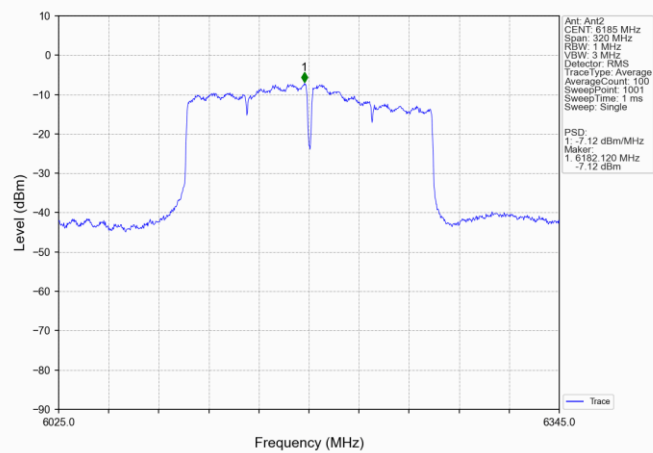
802.11ac(VHT160) MCH_6185MHz_MIMO_NTNV
