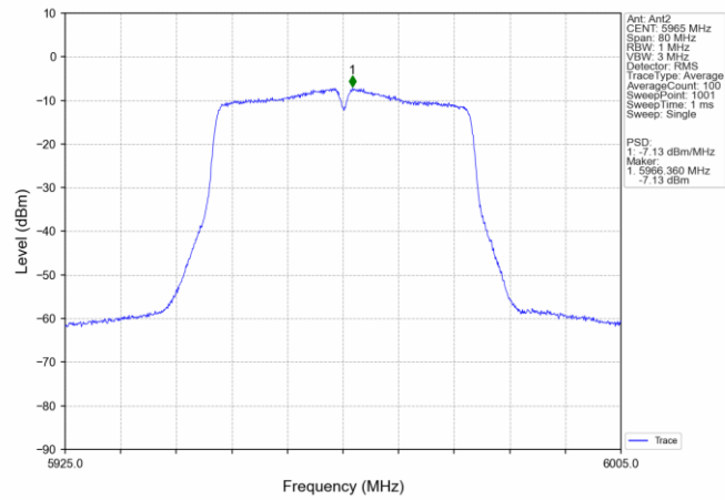
802.11ac(VHT40)_LCH_5965MHz_MIMO_NTNV
