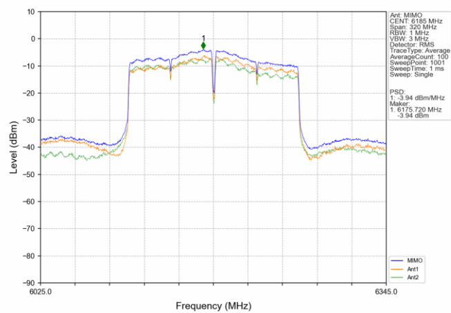
802.11ac(VHT160) MCH_6185MHz_MIMO_NTNV
