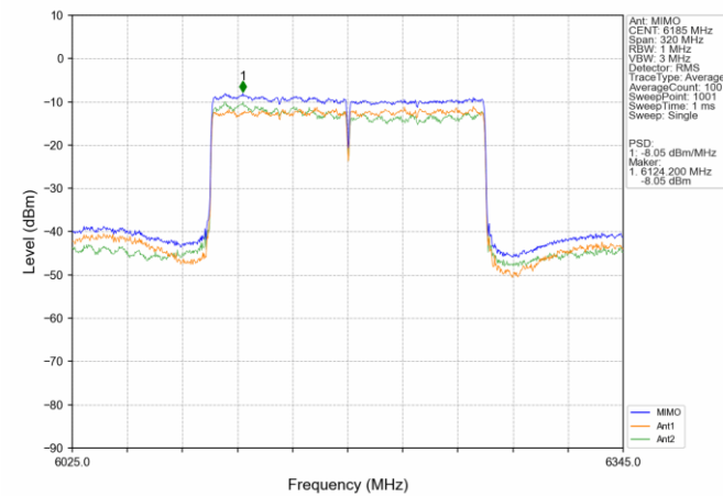
802.11ax(HEW160)_MCH_6185MHz_SU_ / MIMO_NTNV
