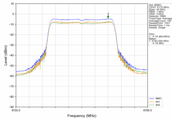
802.11ax(HEW20)_MCH_6175MHz_SU / MIMO NTN
