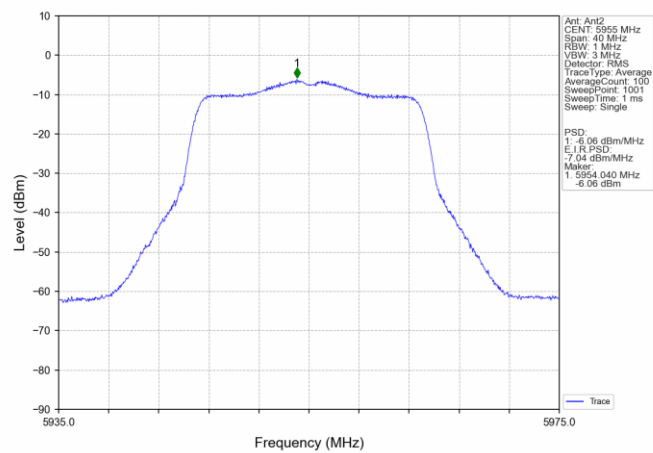
802.11n(HT20)_LCH_5955MHz_MIMO_NTNV
