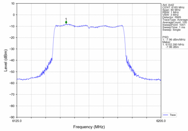
802.11ax(HEW40)_MCH_6165MHz_SU / MIMO NTN
