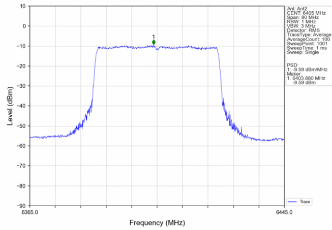
802.11ax(HEW40) HCH_6405MHz_SU / MIMO NTN
