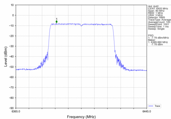
802.11ax(HEW40) HCH_6405MHz_SU / Ant2_NTNV
