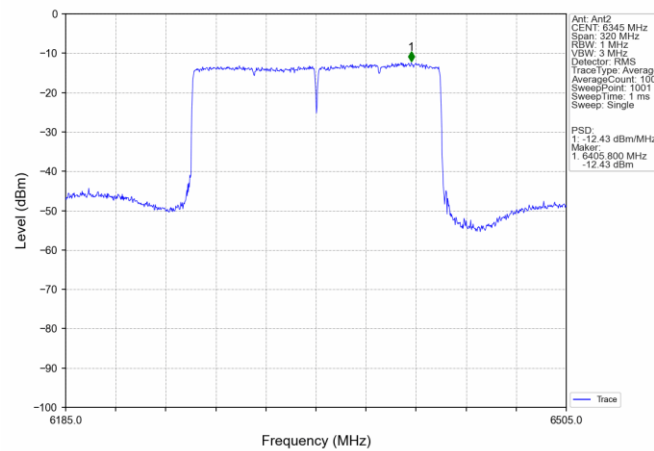
802.11ax(HEW160) HCH 6345MHz_SU / Ant2_NTNV
