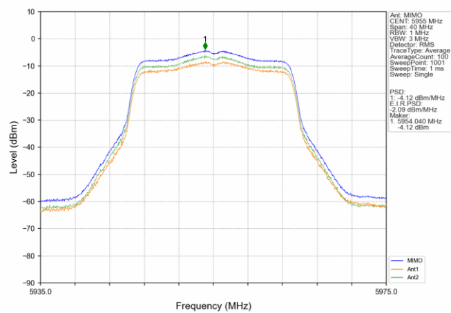
802.11n(HT20)_LCH_5955MHz_MIMO_NTNV
