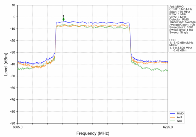
802.11ax(HEW80)_MCH_6145MHz_SU / MIMO NTN
