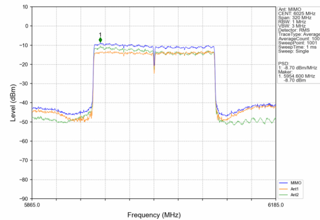
802.11ax(HEW160)_LCH_6025MHz_SU / MIMO NTN
