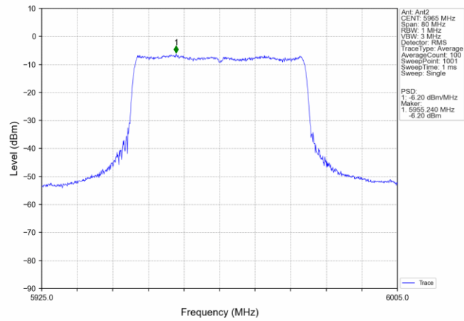
802.11ax(HEW40) LCH_5965MHz_SU / MIMO NTN
