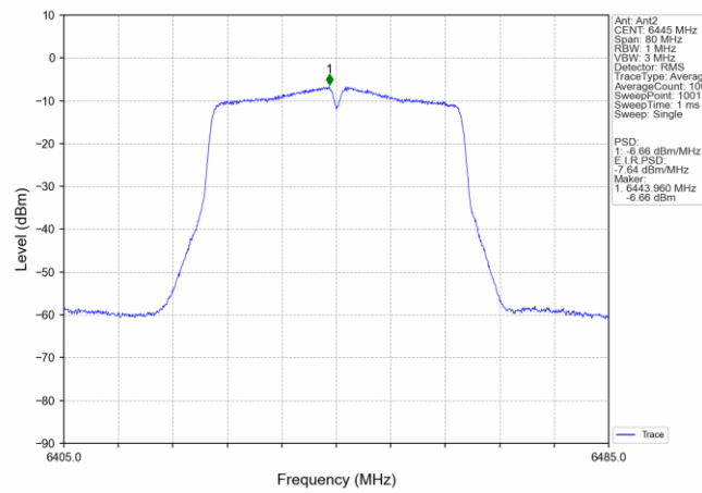
802.11ac(VHT40) LCH 6445MHz Ant2 NTN
