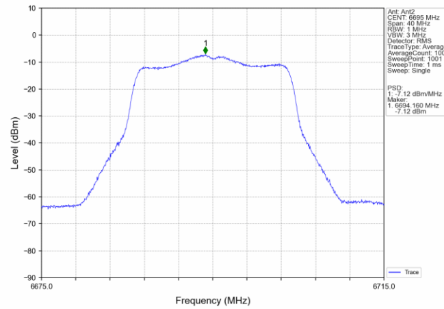
802.11n(HT20) MCH_6695MHz_MIMO_NTN
