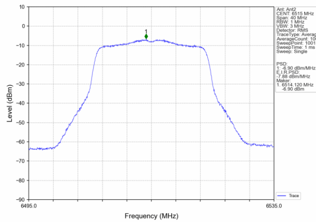
802.11ac(VHT20) HCH_6515MHz_Ant2_NTNV
