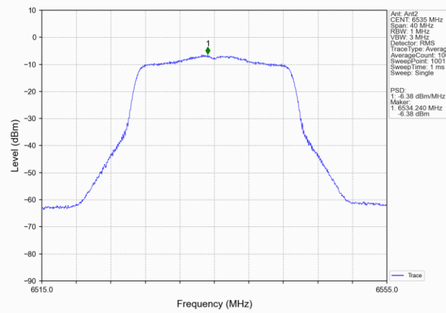
802.11ac(VHT20) LCH_6535MHz_MIMO_NTNV
