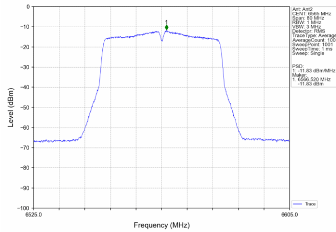
802.11ac(VHT40)_LCH_6565MHz_MIMO_NTNV
