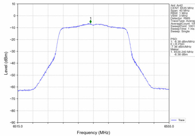
802.11ac(VHT20) LCH_6535MHz_MIMO_NTNV
