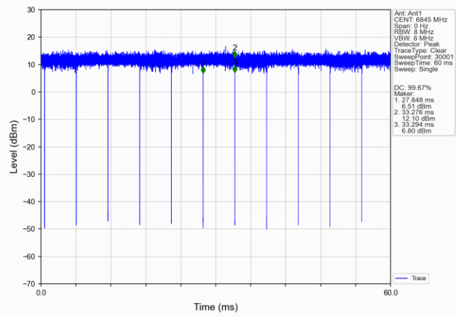
802.11ac(VHT40) HCH_6845MHz_Ant1_NTNV
