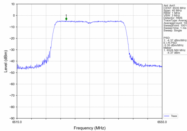
802.11ax(HEW20) LCH_6535MHz_SU_/_Ant1_NTNV
