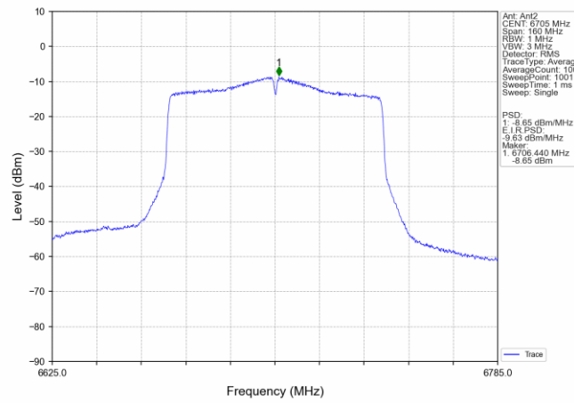
802.11ac(VHT80)_MCH_6705MHz_MIMO_NTNV
