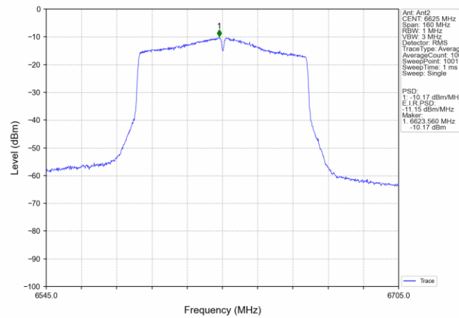
802.11ac(VHT80) LCH_6625MHz_MIMO_NTNV
