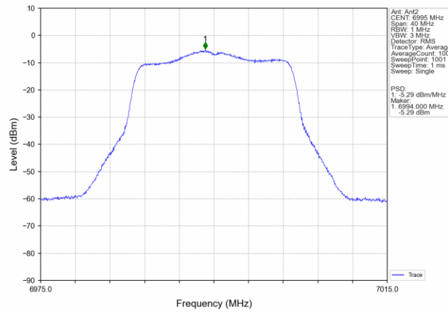
802.11n(HT20) MCH_6995MHz_MIMO_NTN
