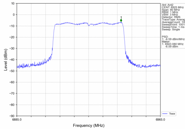
802.11ax(HEW40) LCH_6925MHz_SU_ / MIMO NTN
