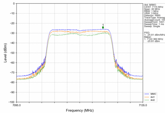
802.11ax(HEW20) HCH_7115MHz_SU / MIMO NTN
