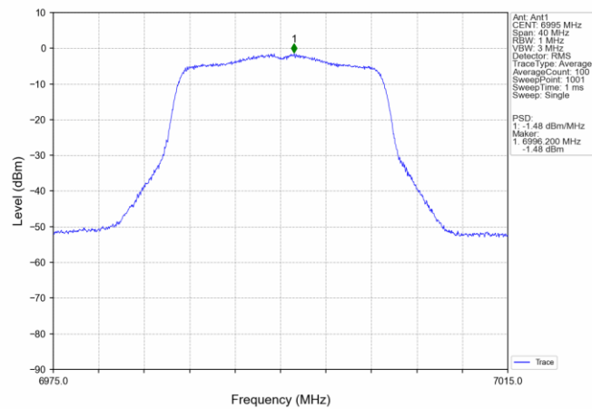
802.11ac(VHT20)_MCH_6995MHz_Ant1_NTNV
