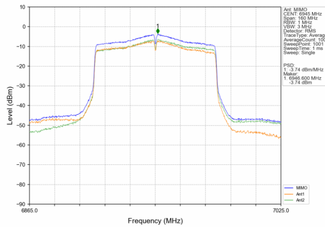
802.11ac(VHT80) LCH_6945MHz_MIMO_NTNV
