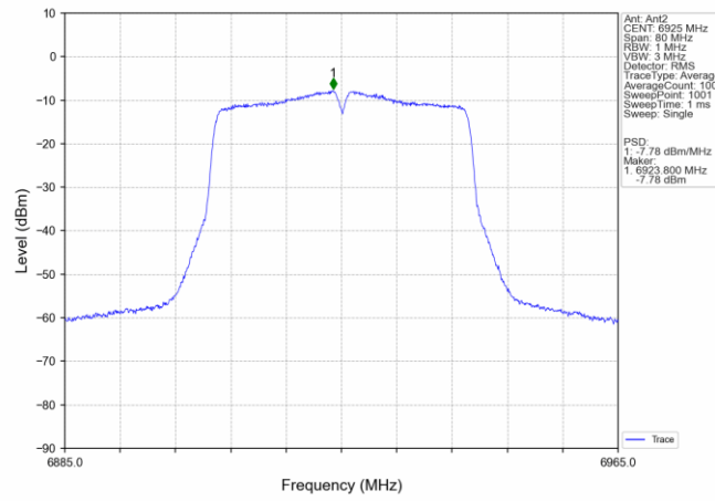
802.11ac(VHT40)_LCH_6925MHz_MIMO_NTNV
