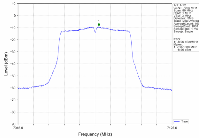
802.11ac(VHT40) HCH_7085MHz_MIMO_NTNV
