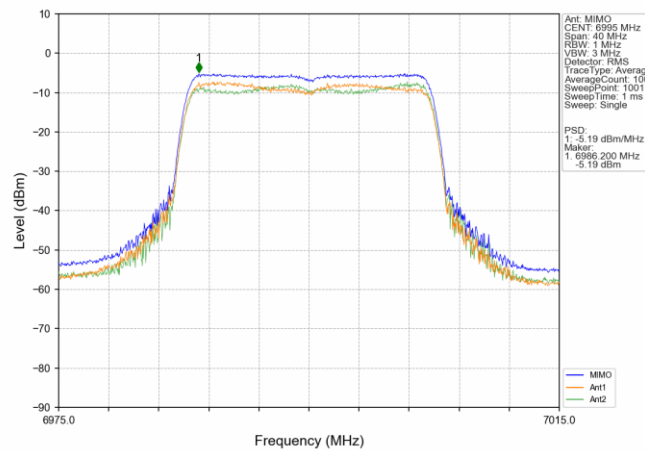
802.11ax(HEW20) MCH_6995MHz_SU / MIMO NTN
