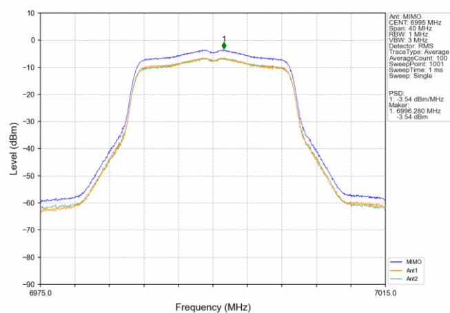
802.11ac(VHT20) MCH_6995MHz_MIMO_NTNV
