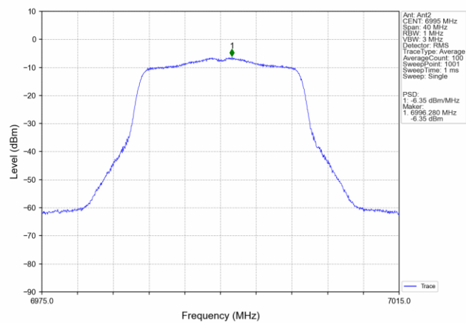
802.11ac(VHT20) MCH_6995MHz_MIMO_NTNV
