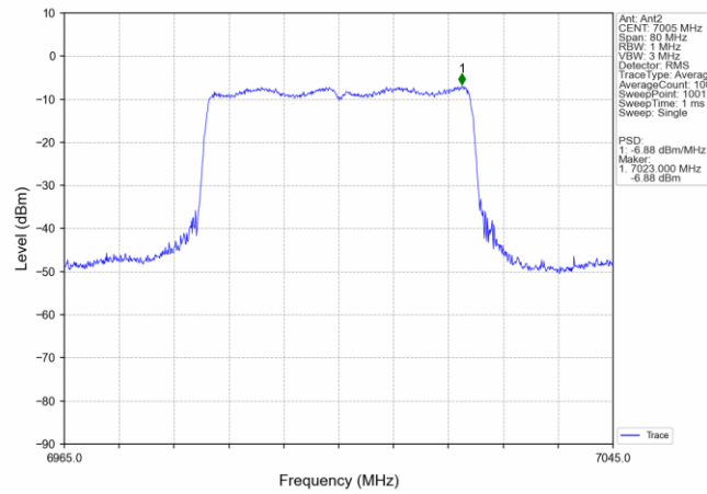
802.11ax(HEW40)_MCH_7005MHz_SU / MIMO NTN
