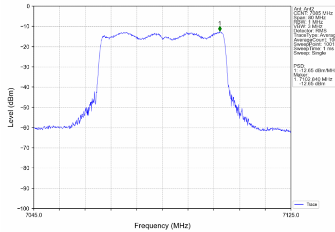
802.11ax(HEW40) HCH_7085MHz_SU / MIMO NTN
