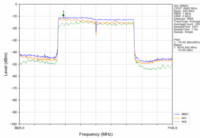
802.11ax(HEW160) MCH_6985MHz_SU / MIMO_NTNV
