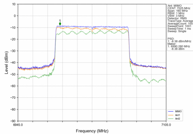
802.11ax(HEW80) HCH_7025MHz_SU / MIMO NTN
