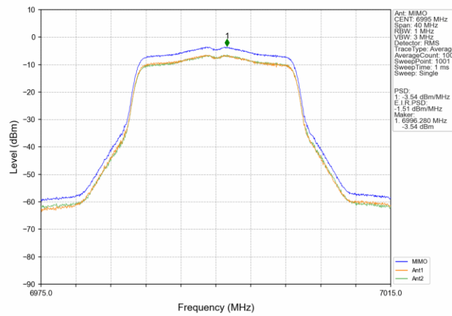
802.11ac(VHT20) MCH_6995MHz_MIMO_NTNV
