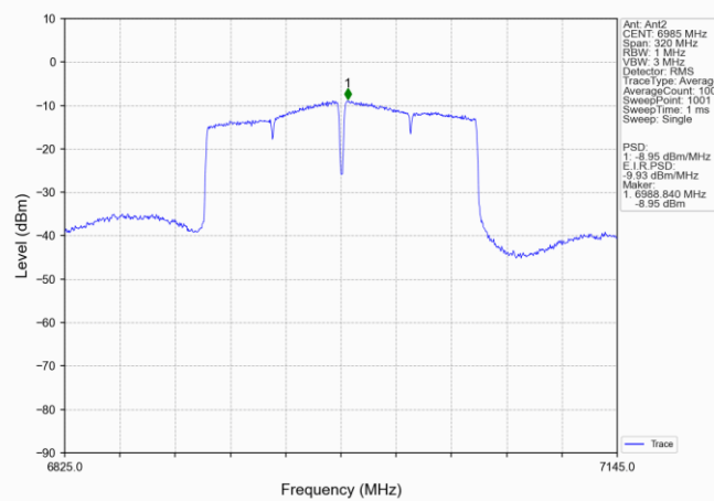
802.11ac(VHT160) MCH_6985MHz_Ant2_NTN
