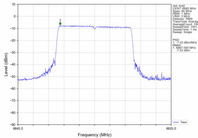
802.11ax(HEW40) HCH_6885MHz_SU / Ant2_NTNV
