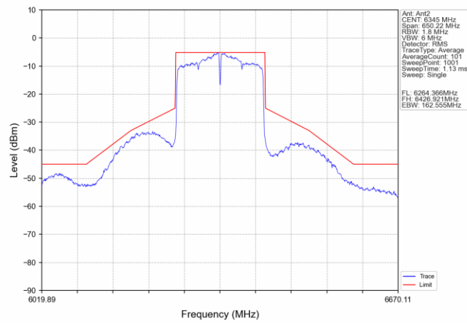
802.11ac(VHT160) HCH_6345MHz_Ant2_NTNV
