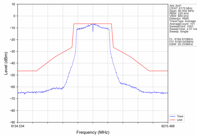
802.11n(HT20) MCH_6175MHz_Ant1_NTNV
