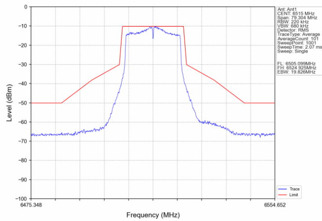
802.11n(HT20) HCH_6515MHz_Ant1_NTN
