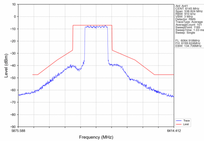
802.11ax(HEW80)_MCH_6145MHz_SU_ / Ant1_NTNV
