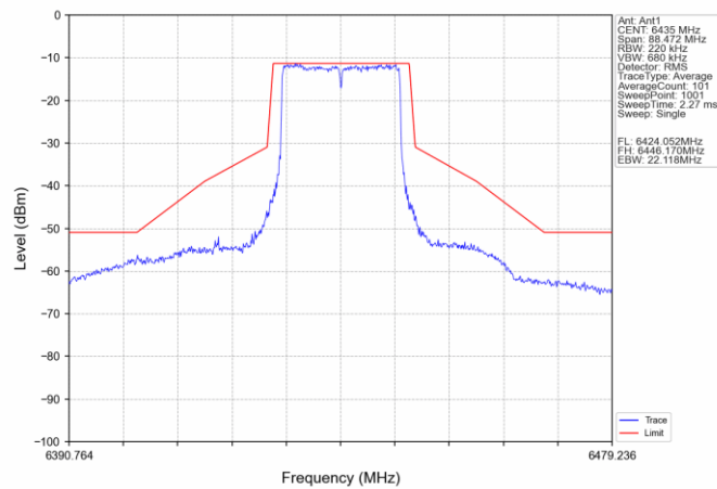
802.11ax(HEW20) LCH_6435MHz_SU_/_Ant1_NTNV
