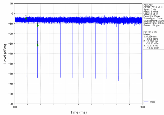
802.11ac(VHT20) HCH_7115MHz_Ant1_NTNV
