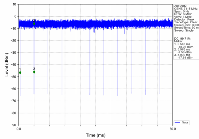
802.11ac(VHT20) HCH_7115MHz_Ant2_NTNV
