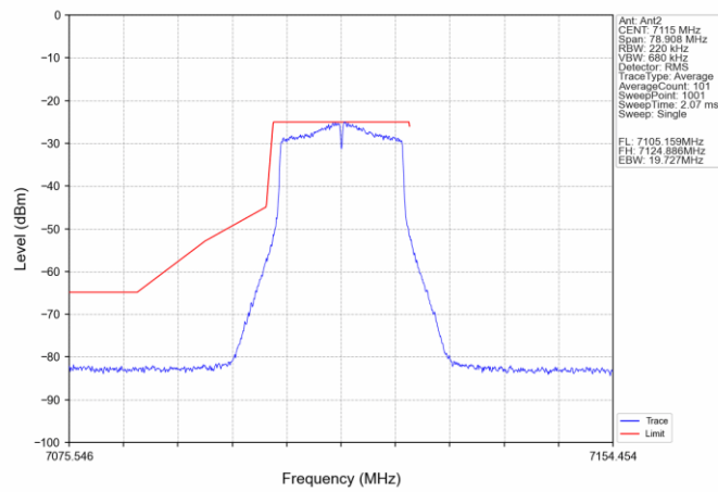
802.11ac(VHT20) HCH_7115MHz_Ant2_NTNV
