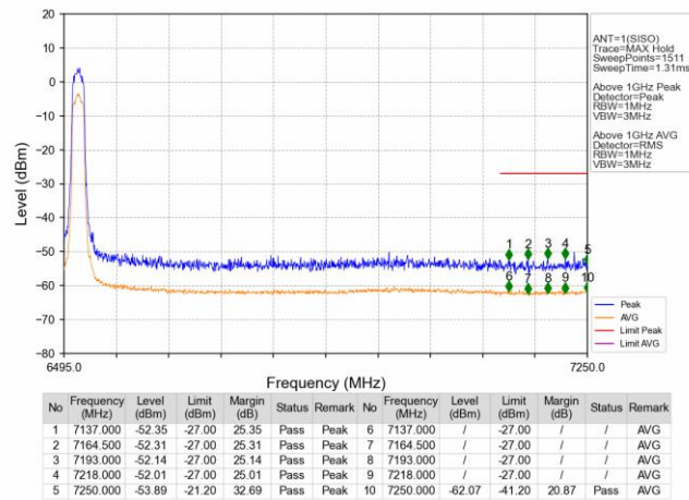
802.11a_HCH_6515MHz_Ant1_NTNV
