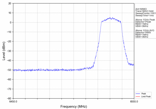
802.11ac(VHT20) LCH_6535MHz_MIMO_NTNV
