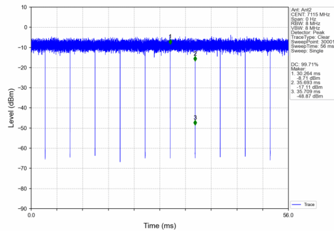
802.11ac(VHT20) HCH_7115MHz_Ant2_NTNV
