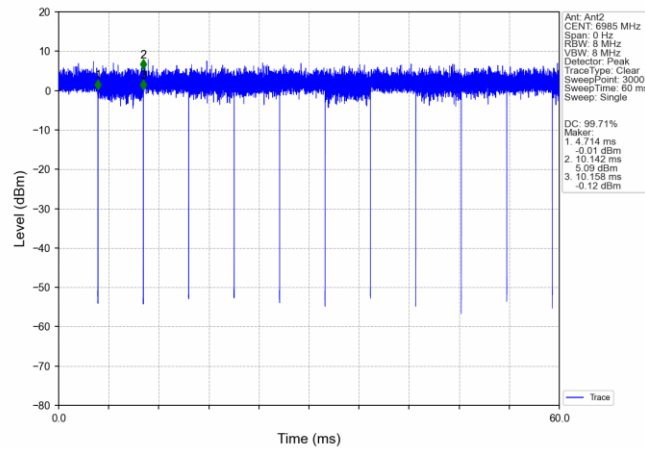
802.11ac(VHT160) MCH_6985MHz_Ant2_NTNV
