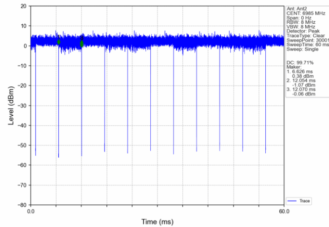
802.11ac(VHT160) MCH_6985MHz_Ant2_NTNV
