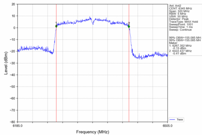
802.11ac(VHT160) HCH_6345MHz_Ant2_NTNV
