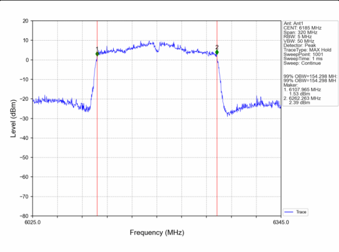
802.11ac(VHT160)_MCH_6185MHz_Ant1_NTNV
