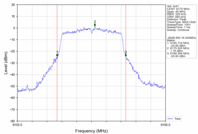
802.11a_MCH_6175MHz_Ant1_NTNV
