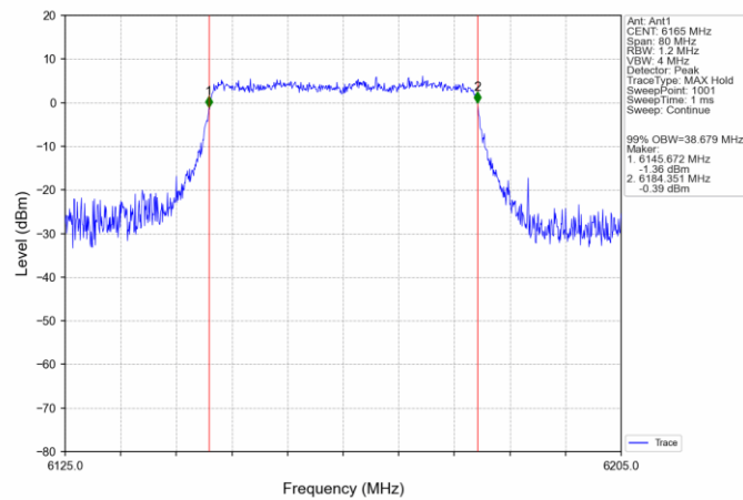
802.11ax(HEW40)_MCH_6165MHz_SU_ / Ant1 NTN
