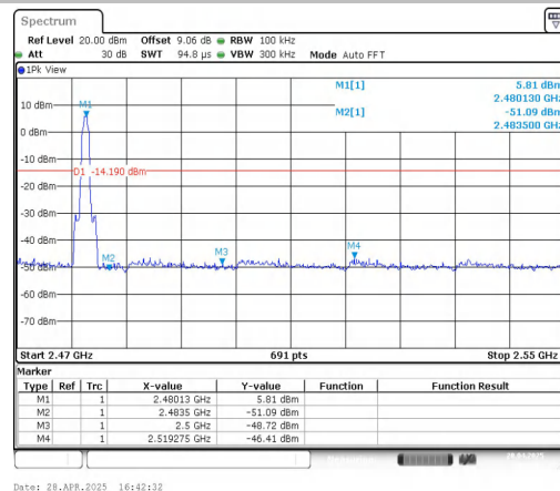
2DH5-Ant1-2480-PASS
