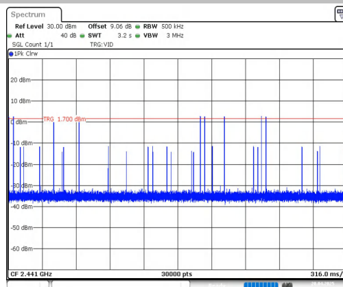
3DH3-Ant1-Hop-PASS
