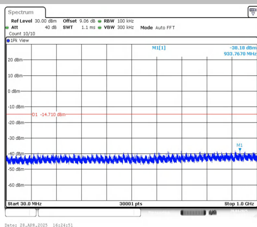
DH5-Ant1-2441-30~1000-PASS
