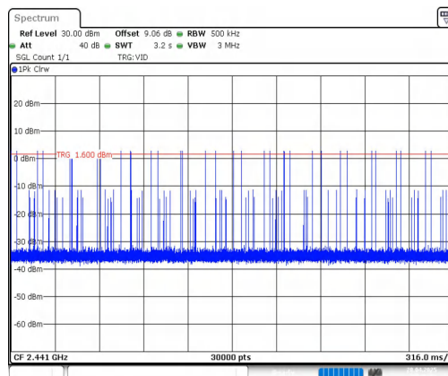
3DH1-Ant1-Hop-PASS
