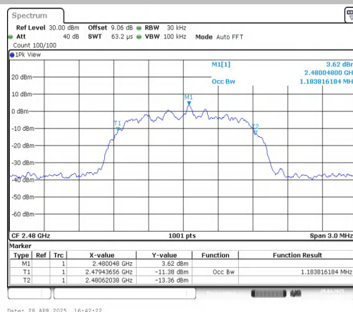
2DH5-Ant1-2480
