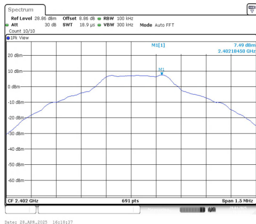
DH5-Ant1-2402-0~Reference-PASS
