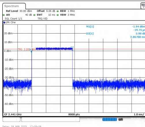
2D3-Ant1-Hop-PASS
