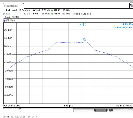
DH5-Ant1-2441-0~Reference-PASS
