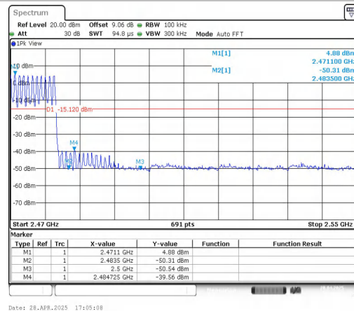
DH5-Ant1-Hop_2480-PASS
