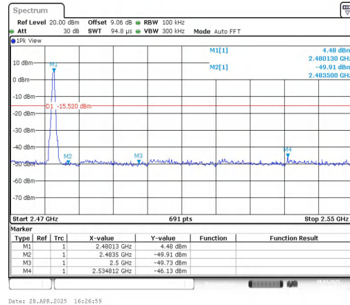
DH5-Ant1-2480-PASS
