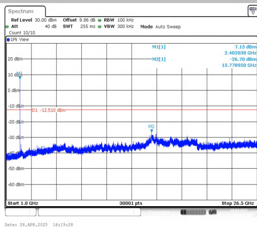
DH5-Ant1-2402-1000~26500-PASS
