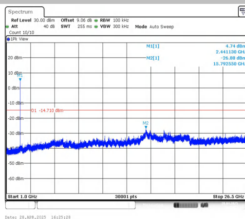
DH5-Ant1-2441-1000~26500-PASS
