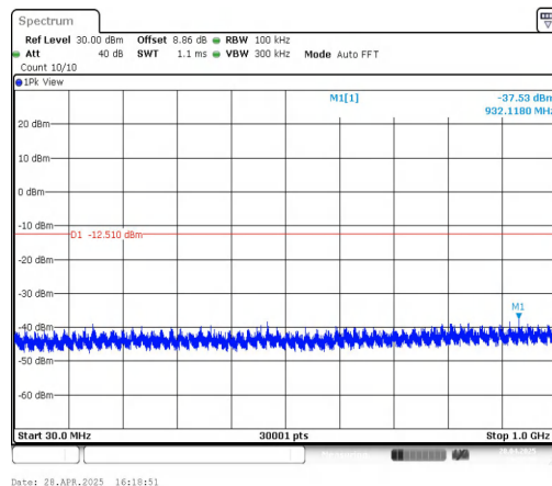
DH5-Ant1-2402-30~1000-PASS
