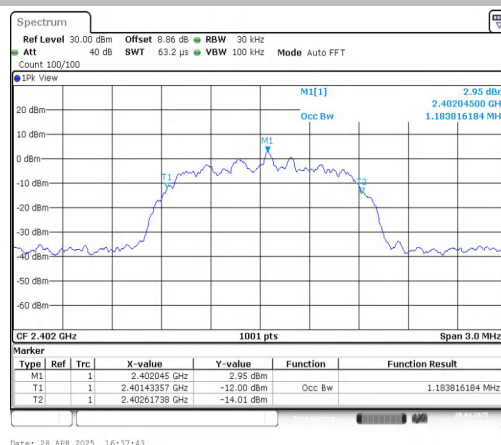
2DH5-Ant1-2402
