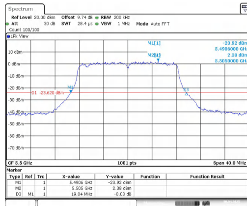
11A-CDD-Ant2-5500
