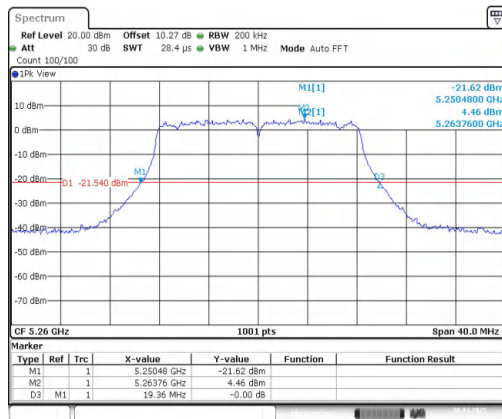
11A-CDD-Ant1-5260
