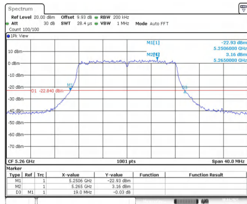
11A-CDD-Ant2-5260
