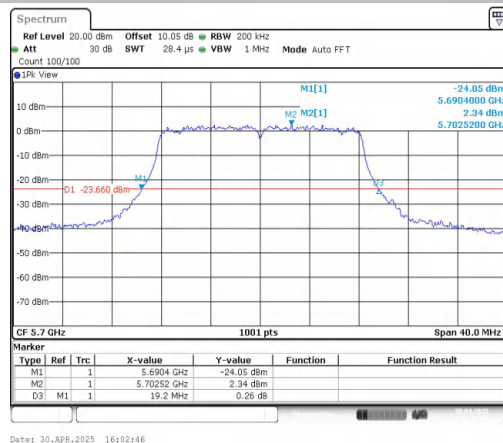
11A-CDD-Ant2-5700
