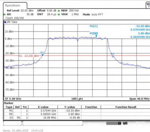
11A-CDD-Ant2-5580
