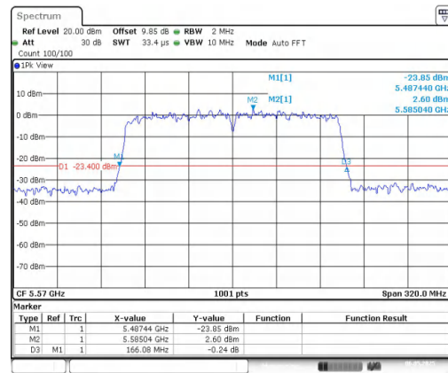
11AC160MIMO-Ant2-5570
