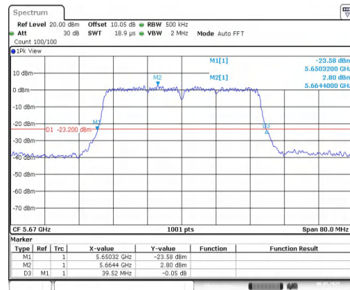
11AC40MIMO-Ant2-5670
