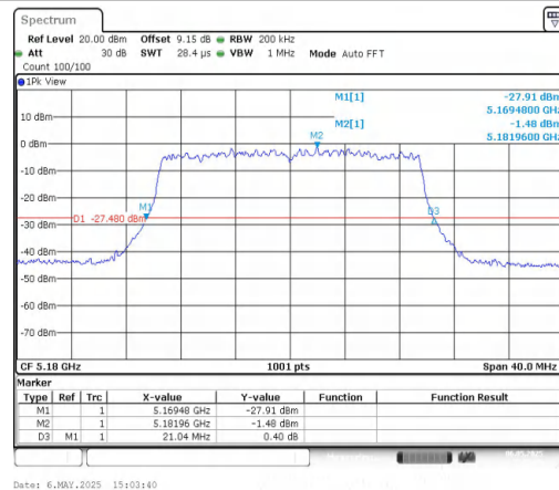
11AX20MIMO-Ant2-5180
