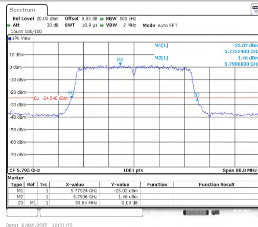
11AC40MIMO-Ant2-5795
