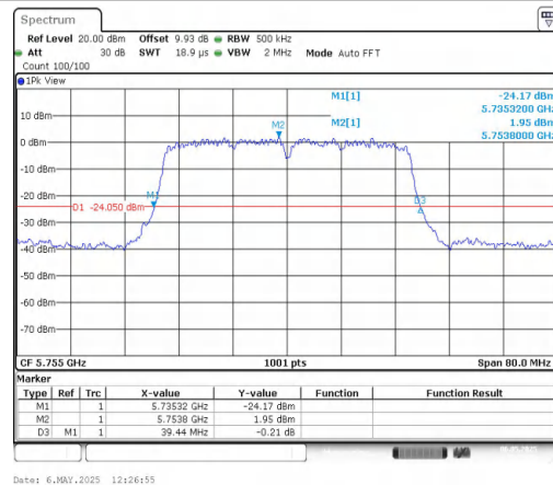
11AC40MIMO-Ant2-5755
