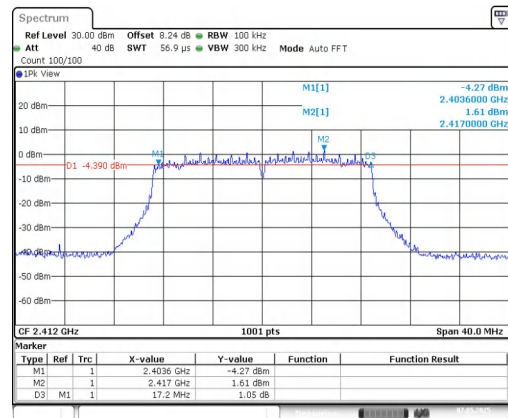
11N20MIMO-Ant2-2412-PASS
