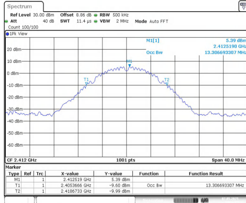
11B-CDD-Ant1-2412
