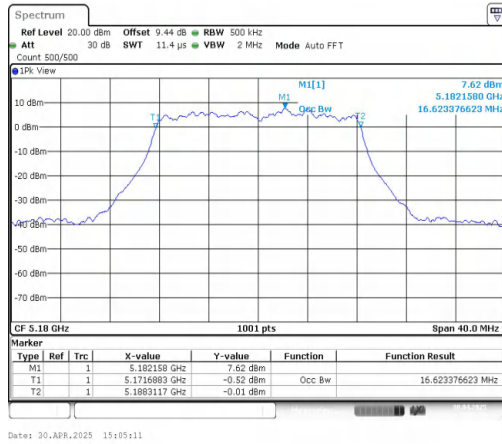
11A-CDD-Ant1-5180
