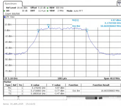
11A-CDD-Ant2-5180
