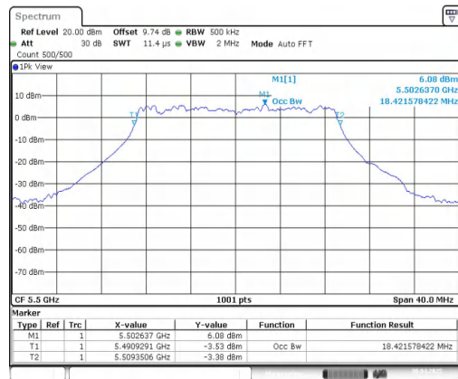
11AC20MIMO-Ant2-5500
