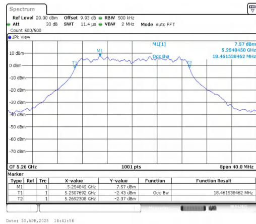
11AC20MIMO-Ant2-5260
