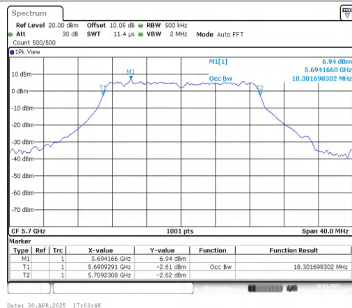
11AC20MIMO-Ant2-5700
