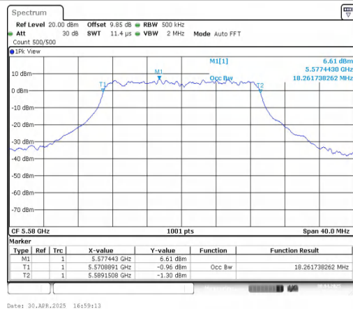
11AC20MIMO-Ant2-5580
