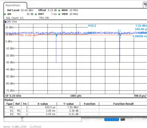
NTNV-11AC40MIMO-Ant2-5230
