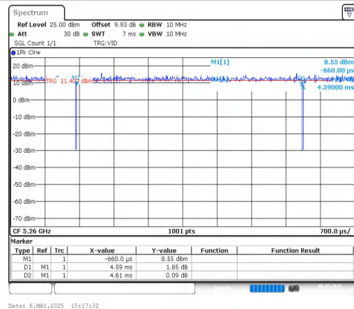
NTNV-11AX20MIMO-Ant2-5260
