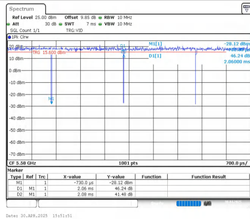
NTNV-11A-CDD-Ant2-5580
