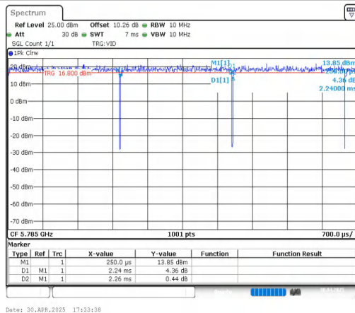
NTNV-11AC20MIMO-Ant1-5785
