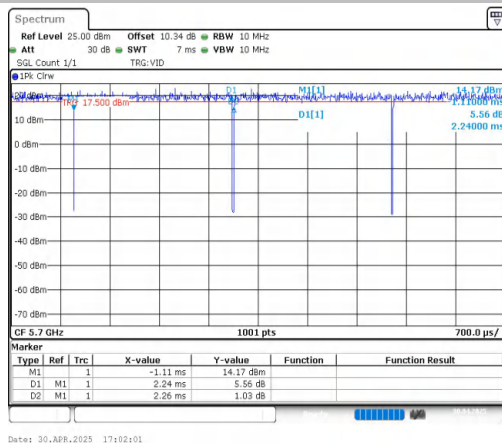
NTNV-11AC20MIMO-Ant1-5700
