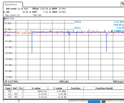
NTNV-11AC160MIMO-Ant2-5570
