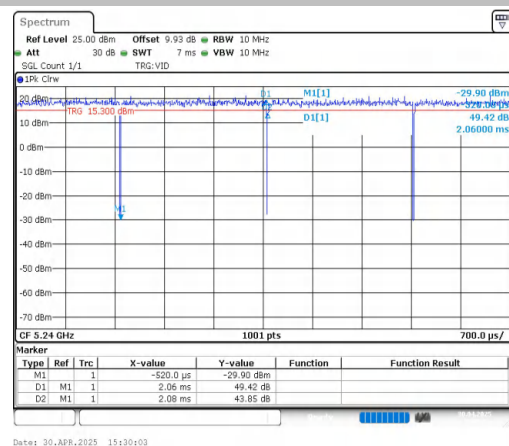
NTNV-11A-CDD-Ant2-5240
