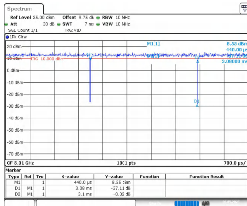
NTNV-11AC40MIMO-Ant1-5310
