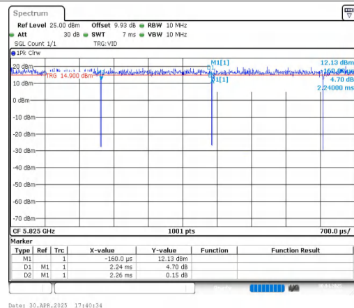
NTNV-11AC20MIMO-Ant2-5825
