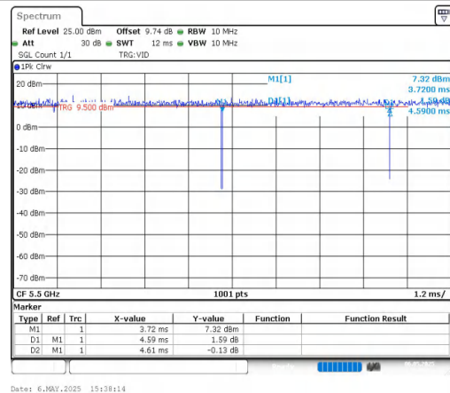
NTNV-11AX20MIMO-Ant2-5500
