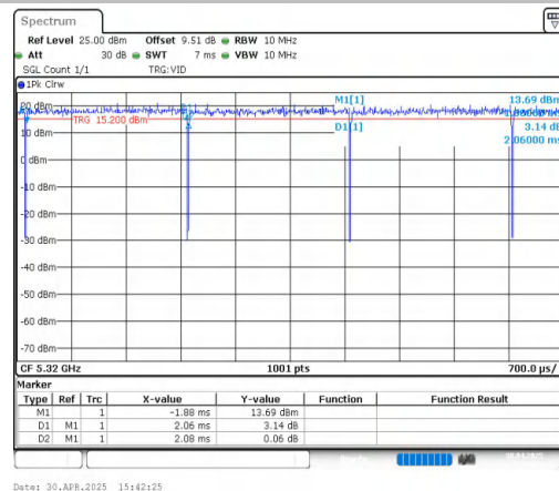
NTNV-11A-CDD-Ant2-5320
