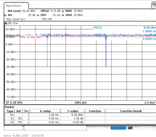
NTNV-11AX20MIMO-Ant2-5180
