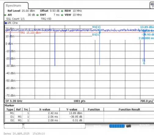
NTNV-11A-CDD-Ant2-5280
