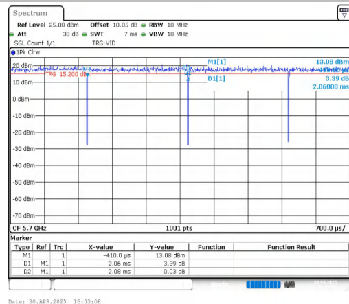
NTNV-11A-CDD-Ant2-5700
