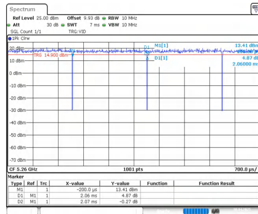
NTNV-11A-CDD-Ant2-5260
