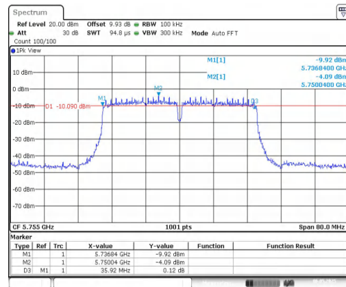
11AC40MIMO-Ant2-5755-PASS
