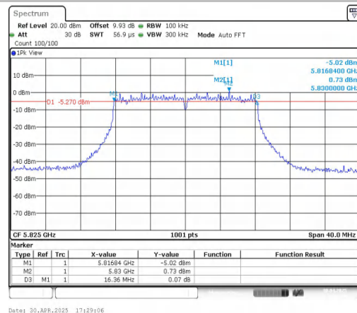
11A-CDD-Ant2-5825-PASS
