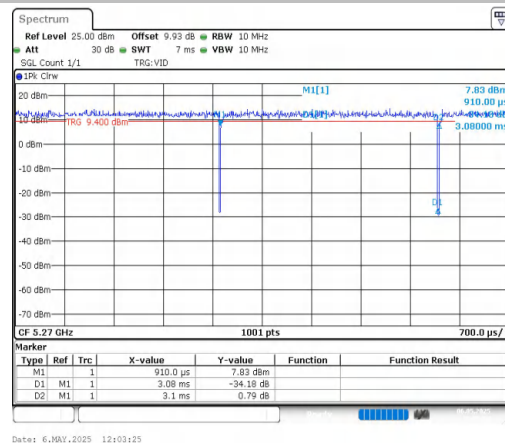
NTNV-11AC40MIMO-Ant2-5270
