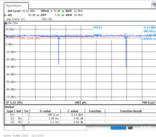
NTNV-11AC40MIMO-Ant2-5510
