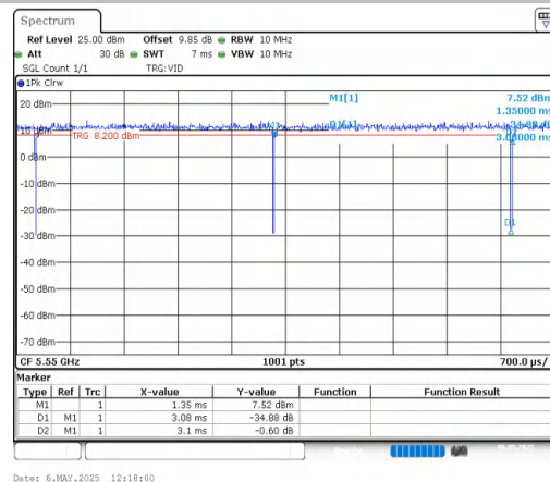
NTNV-11AC40MIMO-Ant2-5550
