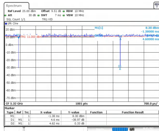
NTNV-11AX20MIMO-Ant2-5320
