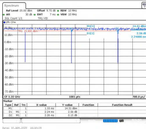
NTNV-11AC20MIMO-Ant1-5320
