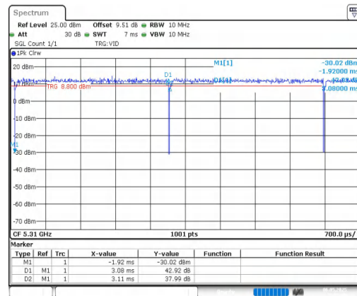
NTNV-11AC40MIMO-Ant2-5310
