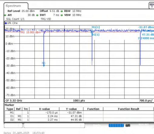
NTNV-11AC20MIMO-Ant2-5320
