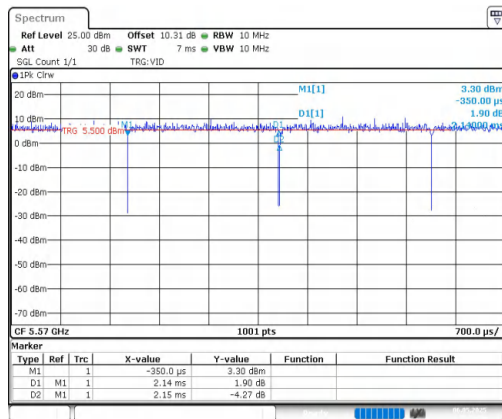
NTNV-11AC160MIMO-Ant1-5570
