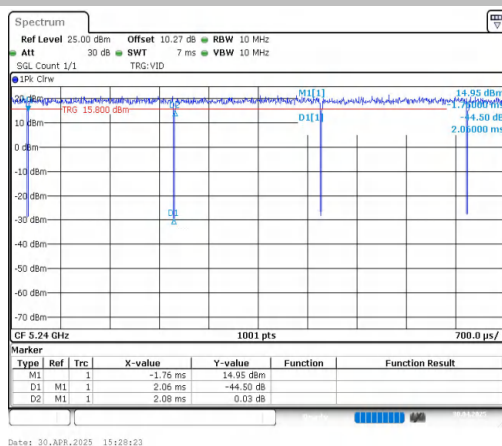
NTNV-11A-CDD-Ant1-5240
