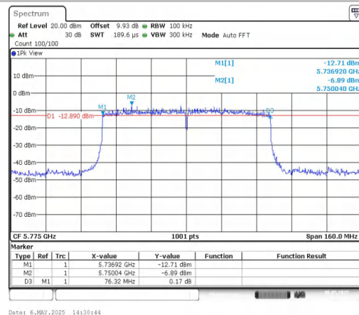
11AC80MIMO-Ant2-5775-PASS
