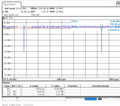
NTNV-11AX20MIMO-Ant1-5180
