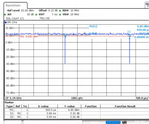
NTNV-11AC40MIMO-Ant2-5190
