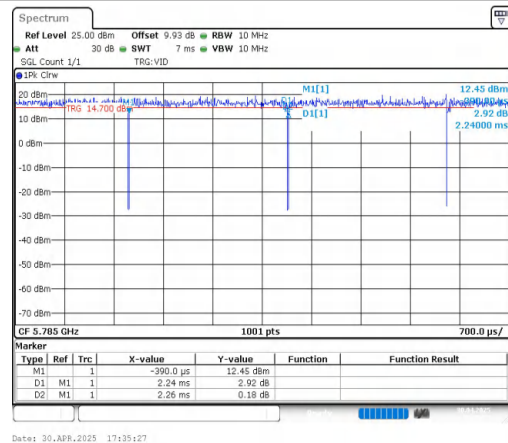
NTNV-11AC20MIMO-Ant2-5785
