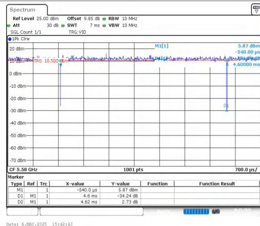
NTNV-11AX20MIMO-Ant2-5580
