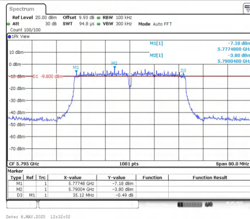
11AC40MIMO-Ant2-5795-PASS
