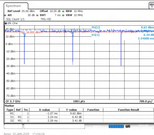
NTNV-11AC20MIMO-Ant2-5700
