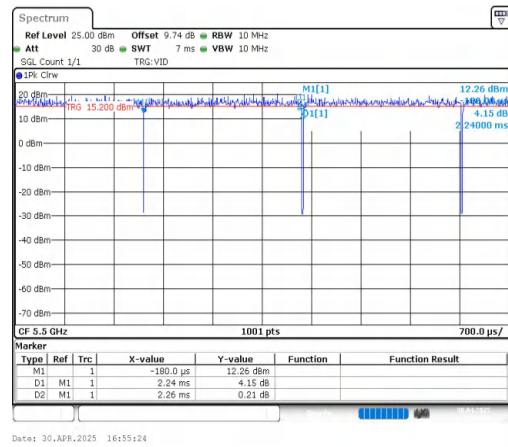
NTNV-11AC20MIMO-Ant2-5500
