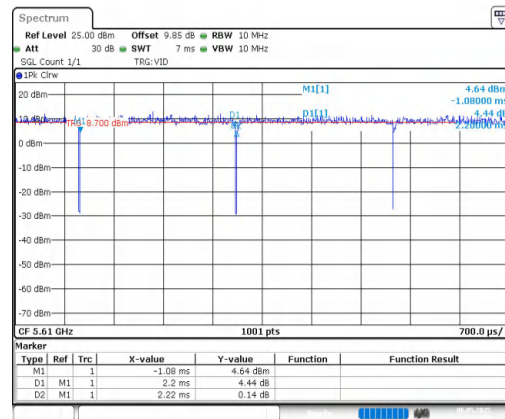
NTNV-11AC80MIMO-Ant2-5610
