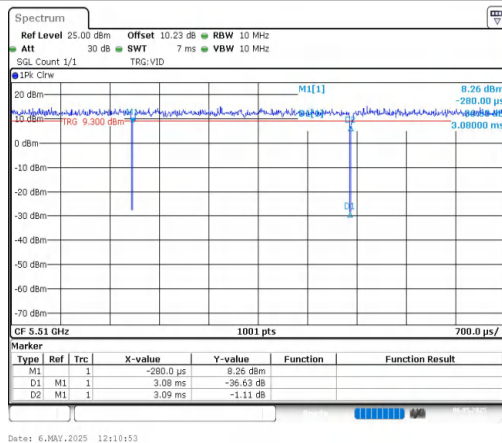
NTNV-11AC40MIMO-Ant1-5510
