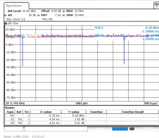
NTNV-11AX20MIMO-Ant2-5745
