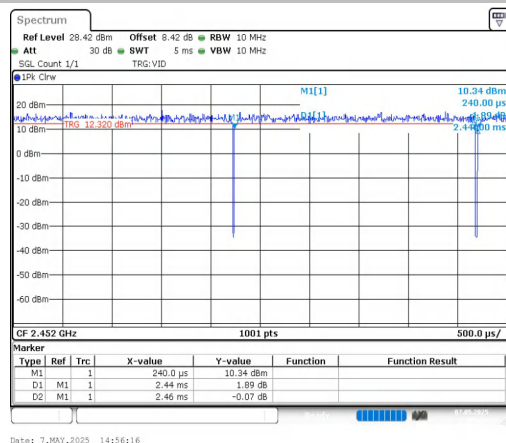
NTNV-11AX40MIMO-Ant2-2452
