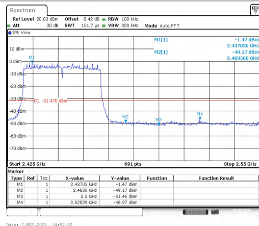
11AX40MIMO-Ant2-2452-PASS
