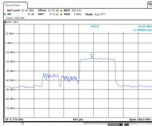
11AX80MIMO-Ant2-5775-484Tone-RU66-PASS
