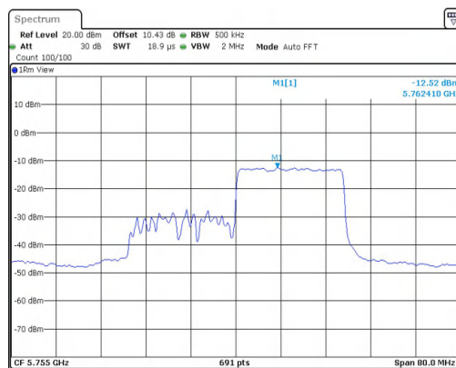
11AX40MIMO-Ant2-5755-242Tone-RU62-PASS
