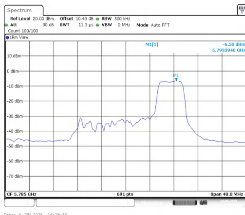
11AX20MIMO-Ant2-5785-52Tone-RU40-PASS
