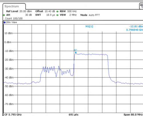
11AX40MIMO-Ant2-5795-242Tone-RU61-PASS
