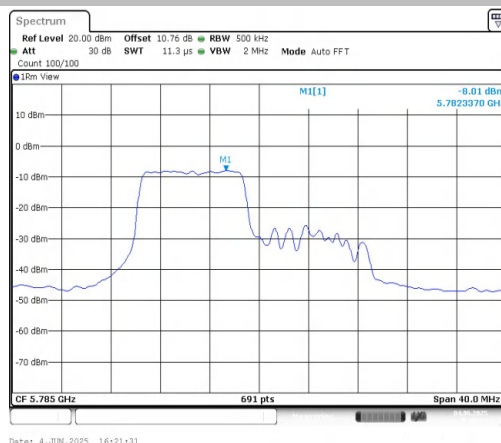
11AX20MIMO-Ant1-5785-106Tone-RU53-PASS
