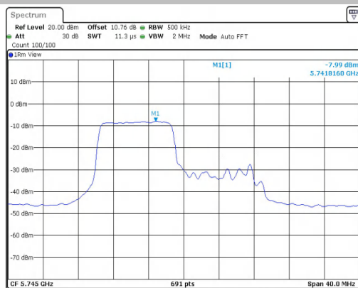
11AX20MIMO-Ant1-5745-52Tone-RU40-PASS
