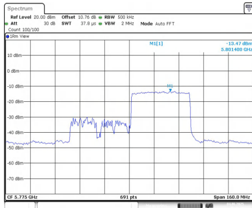
11AX80MIMO-Ant1-5775-484Tone-RU66-PASS
