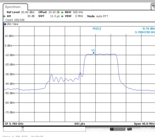
11AX20MIMO-Ant2-5785-106Tone-RU54-PASS
