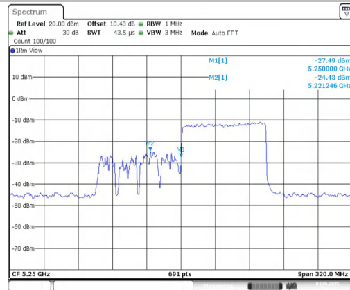
11AX160MIMO-Ant2-5250_UNII-1-996Tone-RU67-PASS
