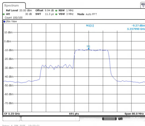
11AX40MIMO-Ant1-5230-242Tone-RU62-PASS
