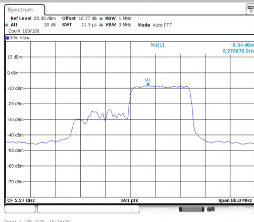
11AX40MIMO-Ant1-5270-242Tone-RU62-PASS
