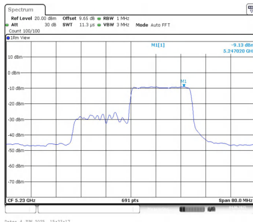
11AX40MIMO-Ant2-5230-242Tone-RU62-PASS
