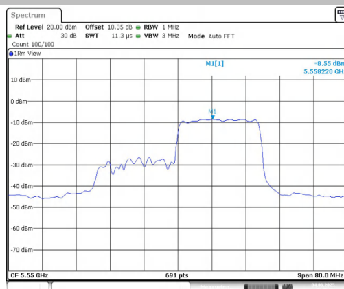
11AX40MIMO-Ant2-5550-242Tone-RU61-PASS
