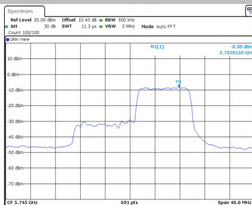
11AX20MIMO-Ant2-5745-106Tone-RU53-PASS
