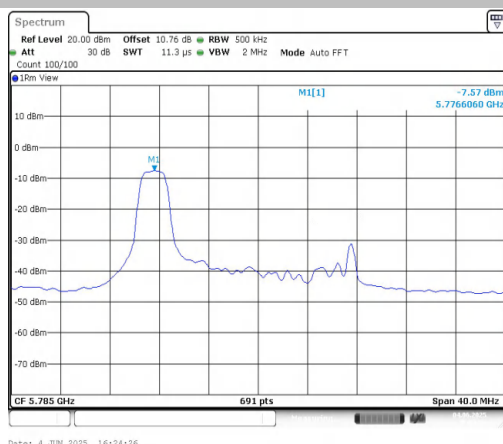
11AX20MIMO-Ant1-5785-106Tone-RU54-PASS
