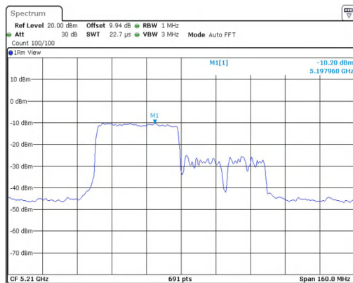
11AX80MIMO-Ant1-5210-484Tone-RU65-PASS
