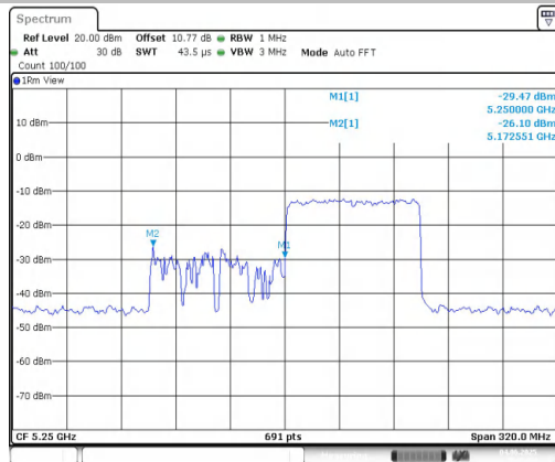
11AX160MIMO-Ant1-5250_UNII-1-996Tone-RU67-PASS
