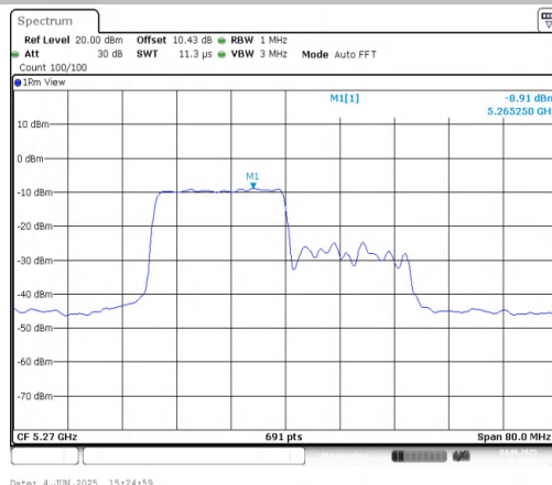
11AX40MIMO-Ant2-5270-242Tone-RU61-PASS
