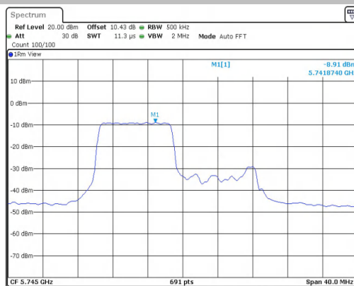
11AX20MIMO-Ant2-5745-52Tone-RU40-PASS
