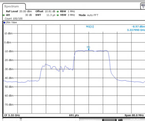
11AX40MIMO-Ant1-5550-242Tone-RU61-PASS
