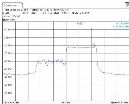
11AX40MIMO-Ant1-5755-242Tone-RU62-PASS
