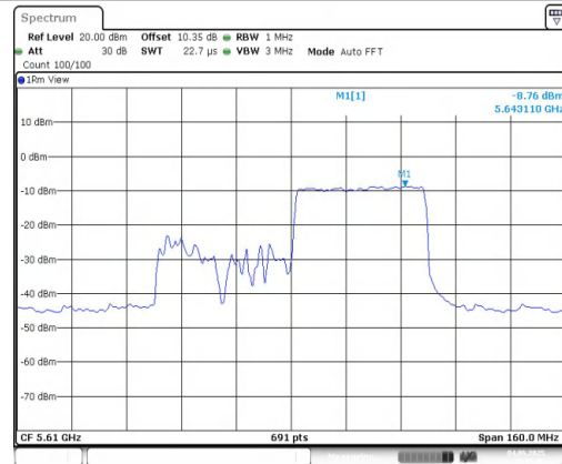
11AX80MIMO-Ant2-5610-484Tone-RU65-PASS
