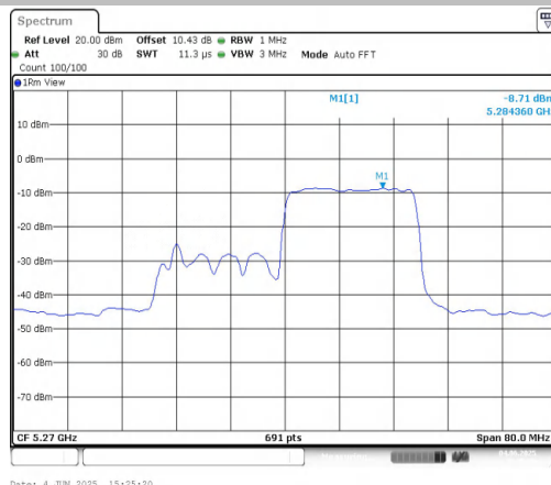
11AX40MIMO-Ant2-5270-242Tone-RU62-PASS
