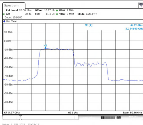
11AX40MIMO-Ant1-5270-242Tone-RU61-PASS
