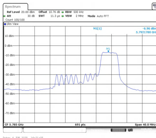
11AX20MIMO-Ant1-5785-52Tone-RU40-PASS
