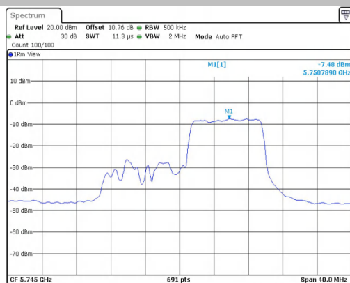
11AX20MIMO-Ant1-5745-106Tone-RU53-PASS
