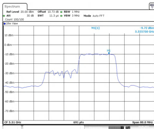
11AX40MIMO-Ant1-5510-242Tone-RU62-PASS
