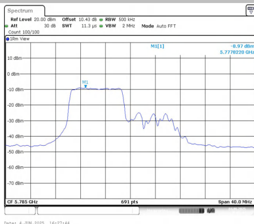
11AX20MIMO-Ant2-5785-106Tone-RU53-PASS
