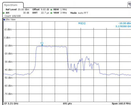
11AX80MIMO-Ant2-5210-484Tone-RU65-PASS
