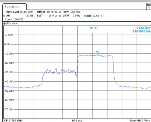
11AX40MIMO-Ant1-5795-242Tone-RU61-PASS
