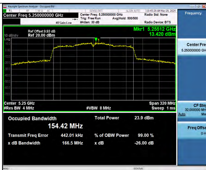
11AC160MIMO Ant2 5250
