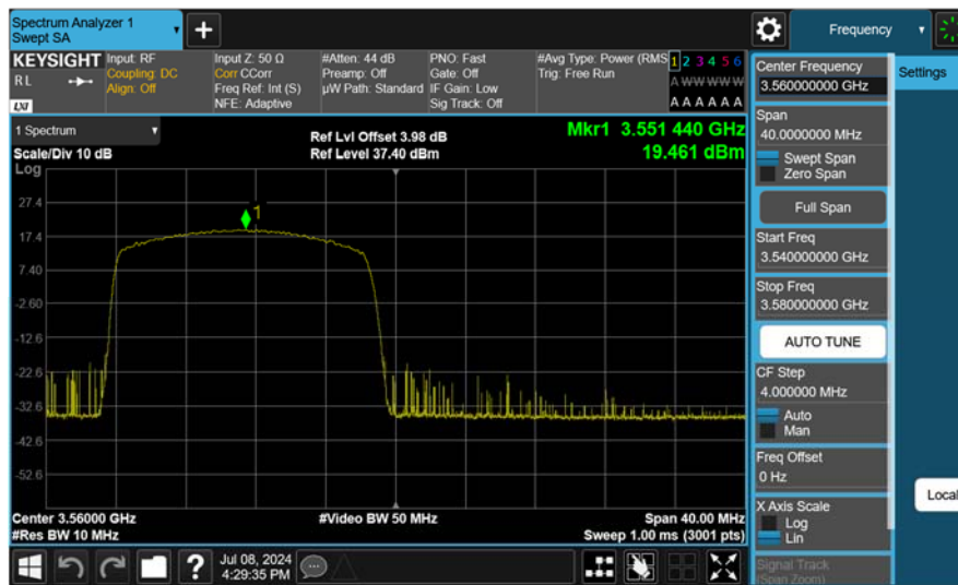
20 MHz / QPSK / RB Size/Offset (1/0) - Low Channel
