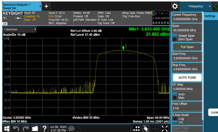
20 MHz / QPSK / RB Size/Offset (1/99) - Middle Channel
