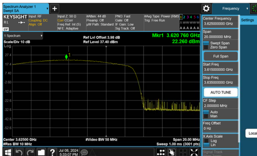
10 MHz / QPSK / RB Size/Offset (1/0) - Middle Channel
