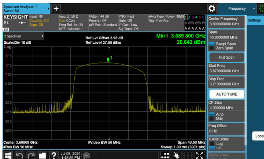
20 MHz / QPSK / RB Size/Offset (1/50) - High Channel
