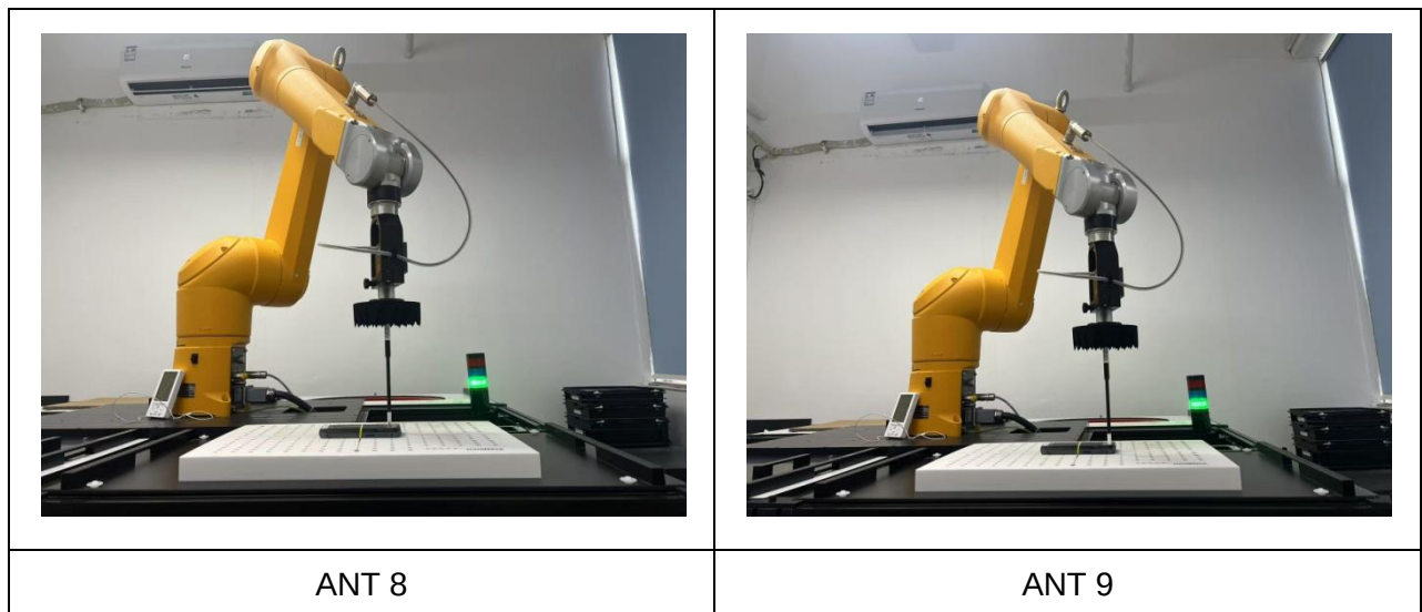
Back Side (Test distance: 2mm)
