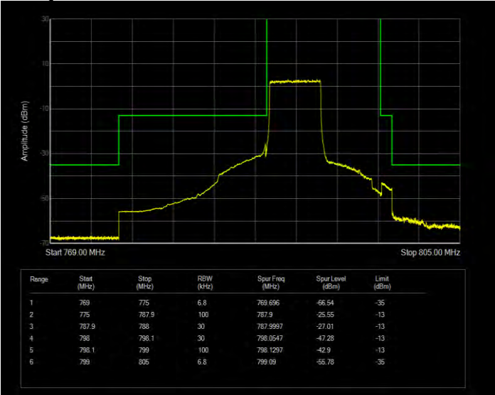
Band14 QPSK BW=5MHz Channel=23305 RB Size=25 Position=#0 Normal
