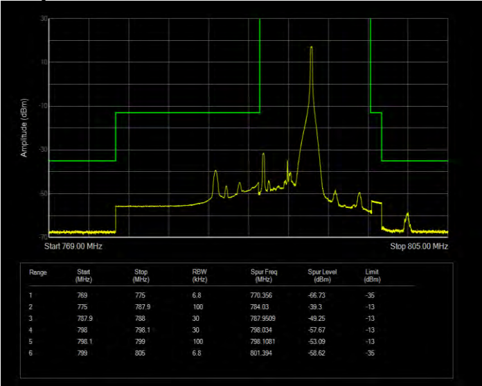
Band14 QPSK BW=5MHz Channel=23305 RB Size=25 Position=#0 Extended
