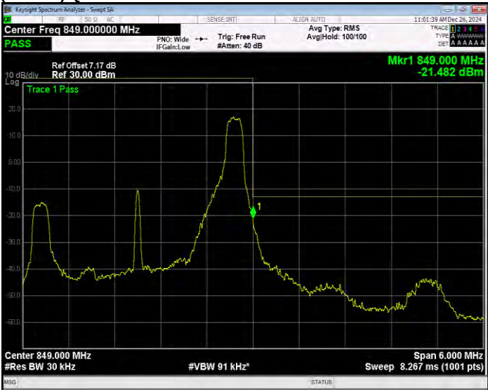
Band26(824-849) QPSK BW=3MHz Channel=27025 RB Size=15 Position=#0 Extended
