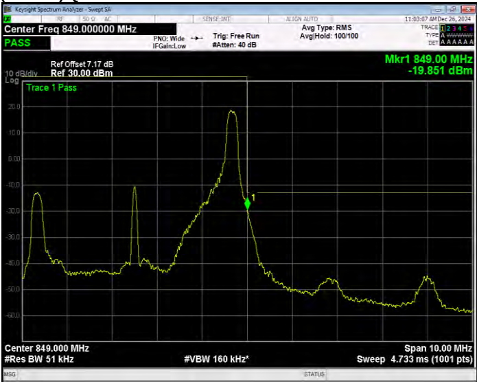
Band26(824-849) QPSK BW=5MHz Channel=27015 RB Size=25 Position=#0 Extended
