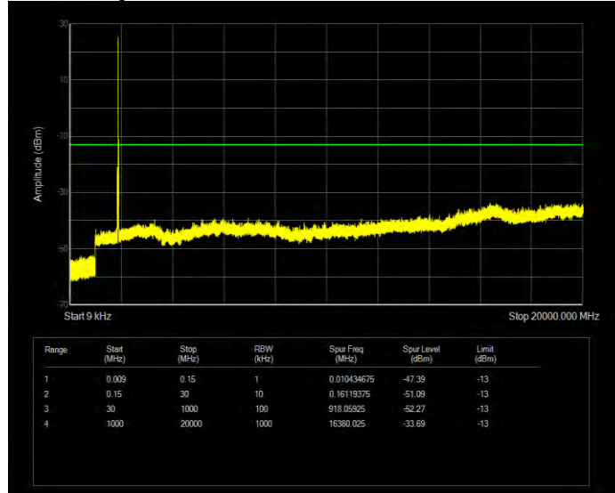
Band25 16QAM BW=3MHz Channel=26055 RB Size=1 Position=#0
