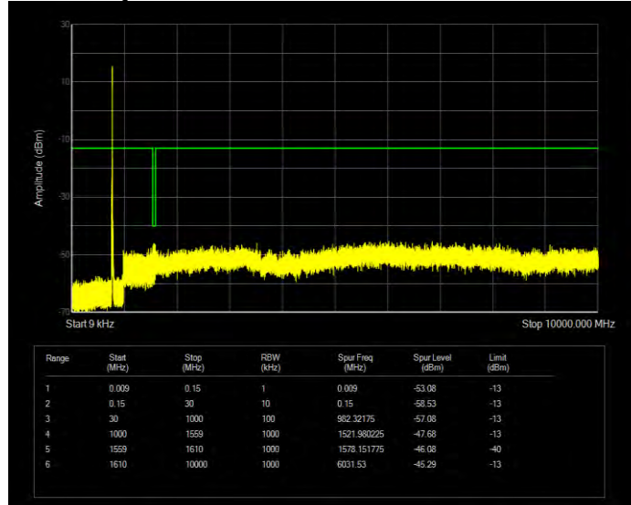
Band14 16QAM BW=5MHz Channel=23330 RB Size=25 Position=#0
