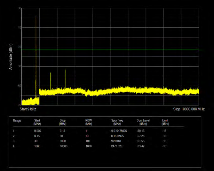
Band26(824-849) 16QAM BW=3MHz Channel=26915 RB Size=1 Position=#0
