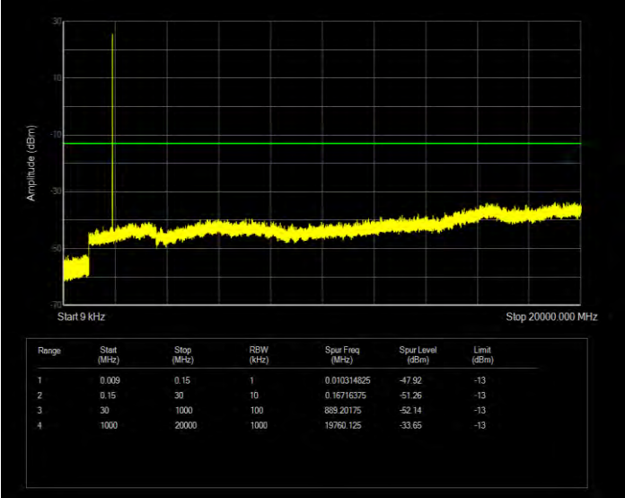
Band25 QPSK BW=5MHz Channel=26065 RB Size=1 Position=#0
