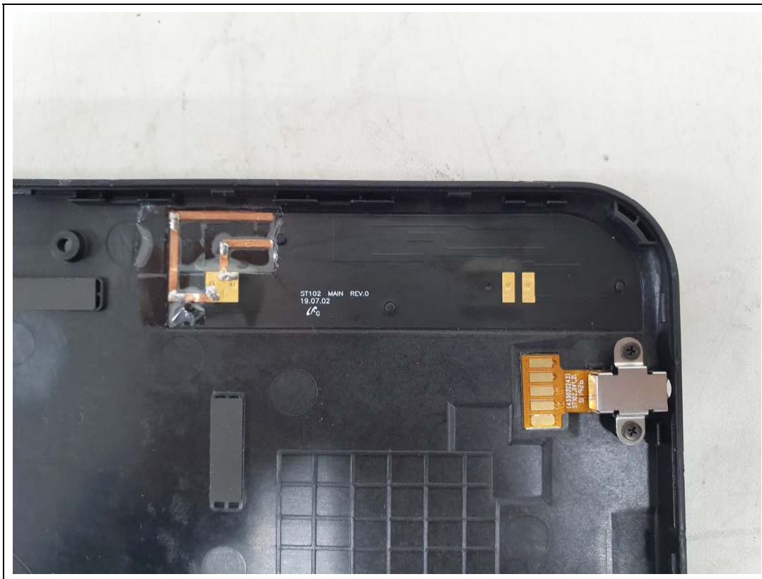
<Main Antenna>
