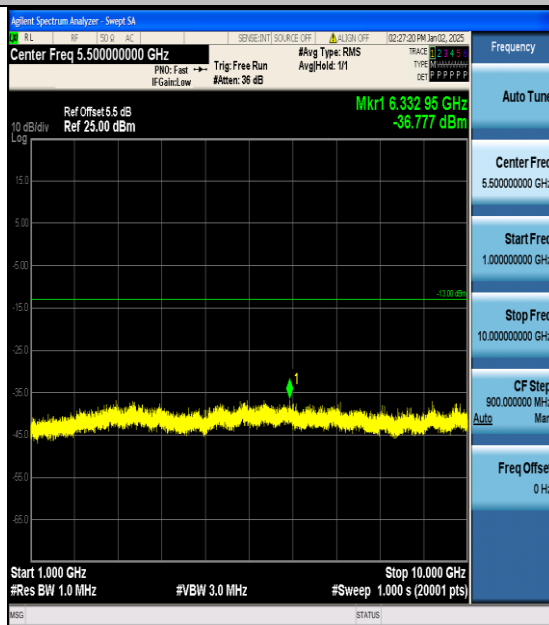
Band5-4132-1-1000~10000MHz-PASS
