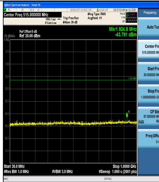
Band4-1513-1-30~1000MHz-PASS
