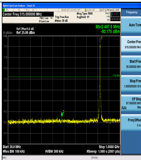
Band5-4132-1-30~1000MHz-PASS
