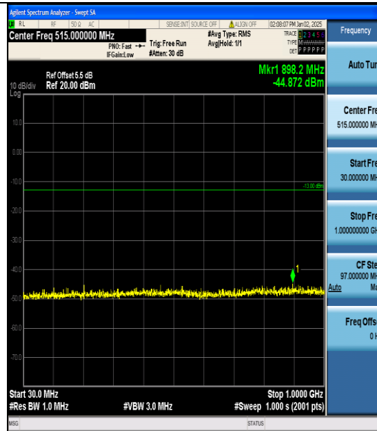
Band2-9262-1-30~1000MHz-PASS
