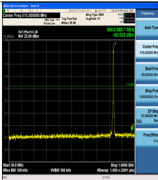
Band5-4182-1-30~1000MHz-PASS
