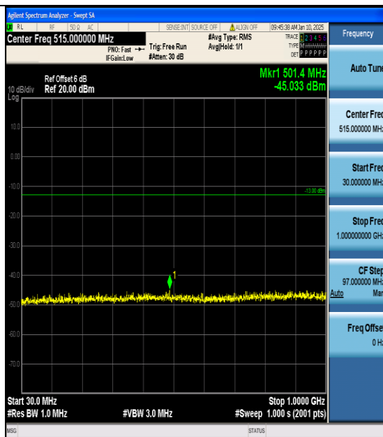
Band4-1513-1-30~1000MHz-PASS
