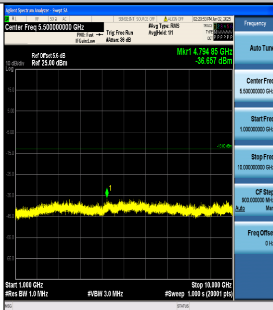
Band5-4182-1-1000~10000MHz-PASS
