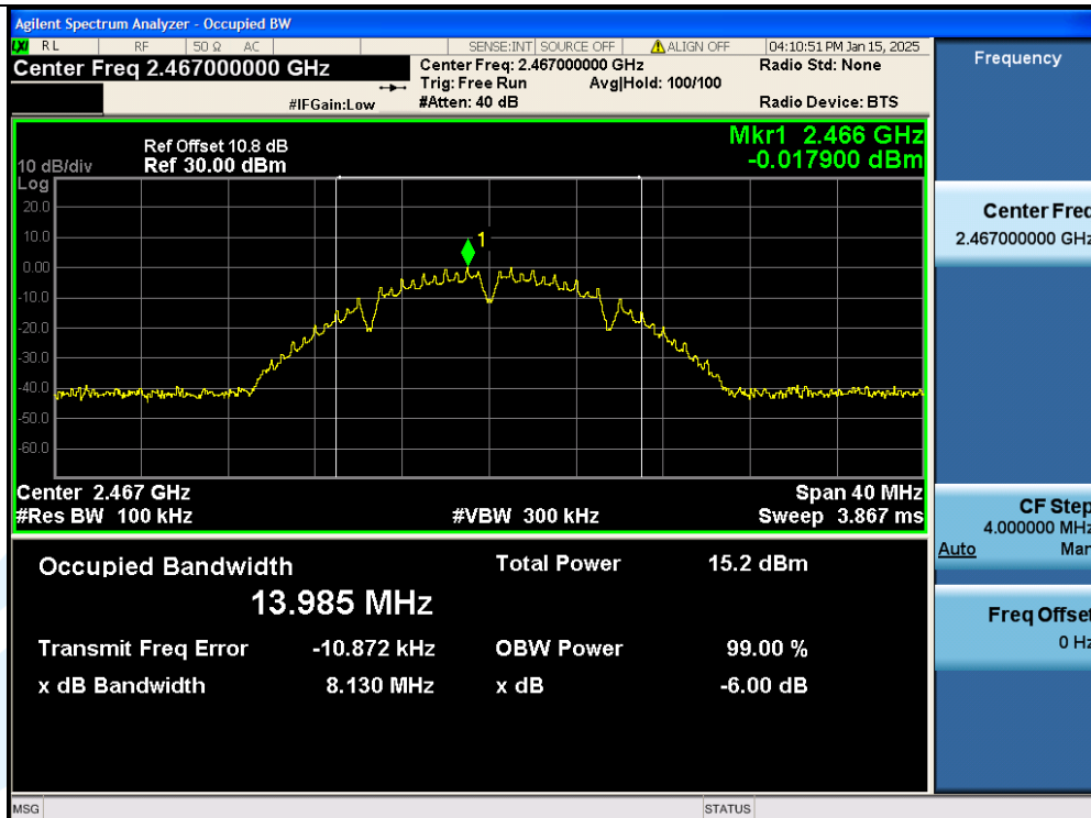
11B-Ant1-2467MHz-PASS
