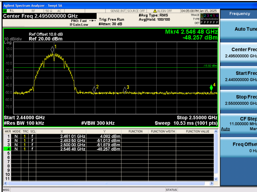
11B-Ant1-2462MHz-PASS
