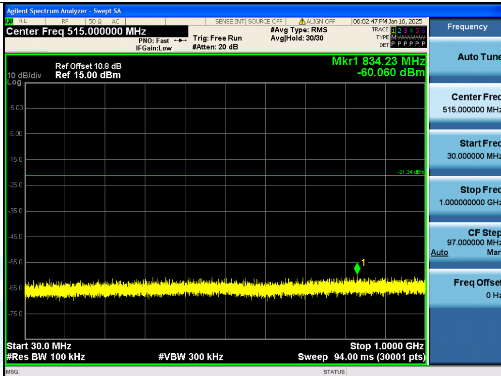
11G-Ant1-2462MHz-30~1000 MHz-PASS
