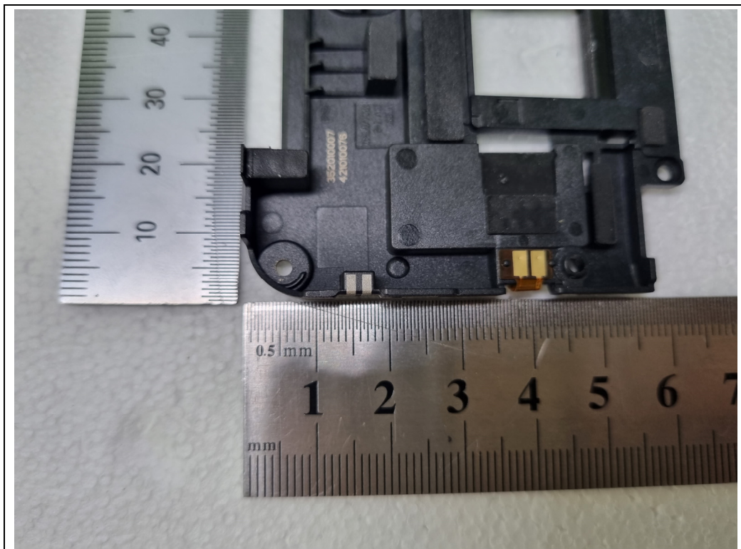
<WIFI Antenna>
