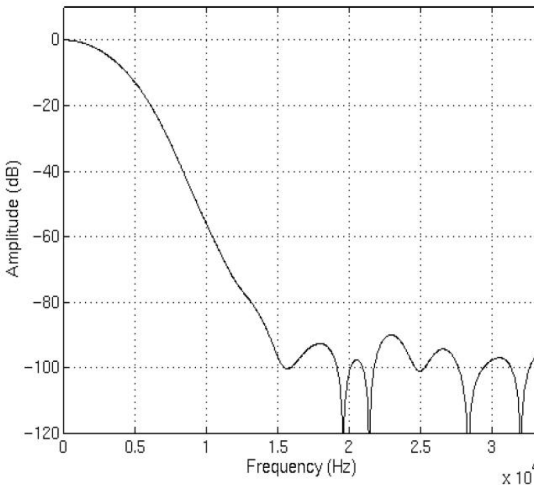
Figure 2. Modulation Filter
