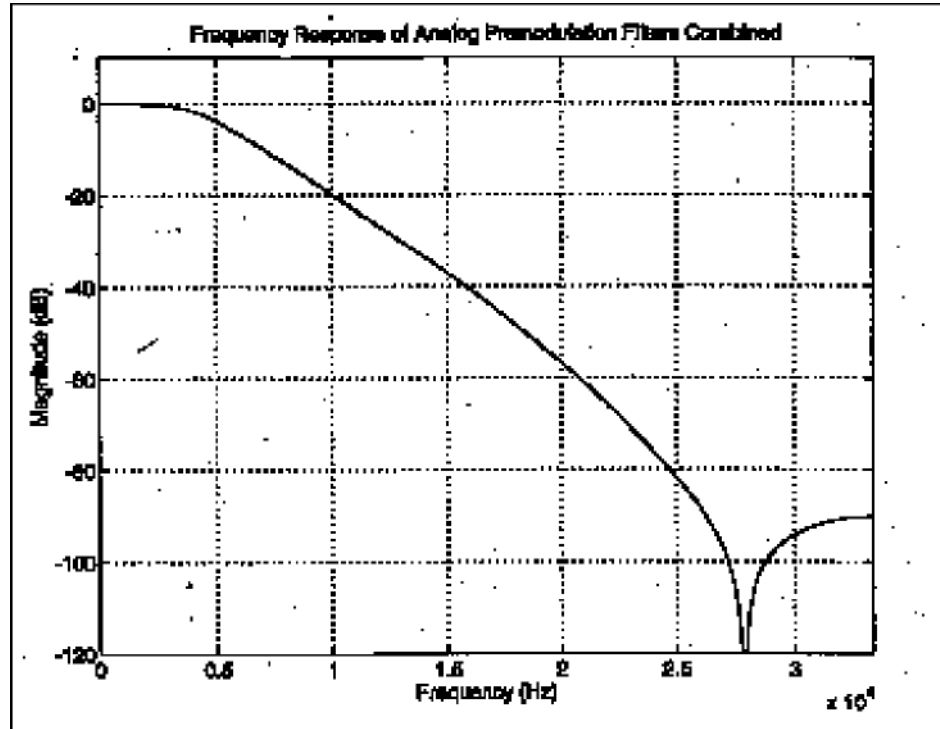
Figure 1. Frequency Response
