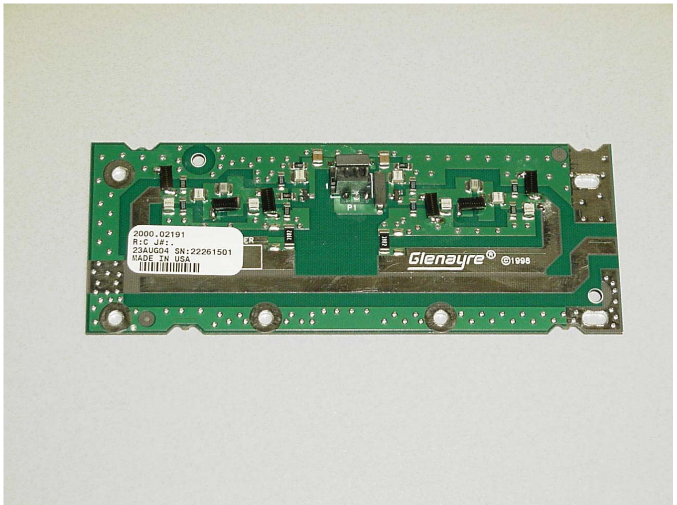
2000.02191 Directional coupler
