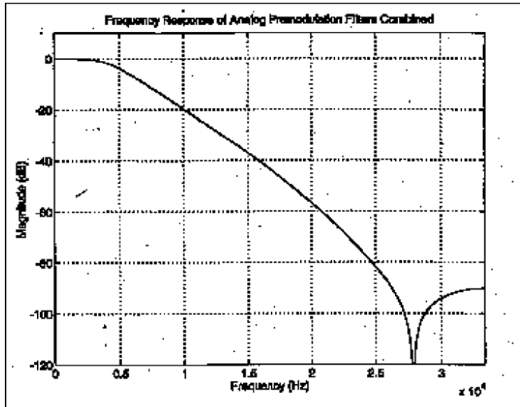
Figure 1. Frequency Response
