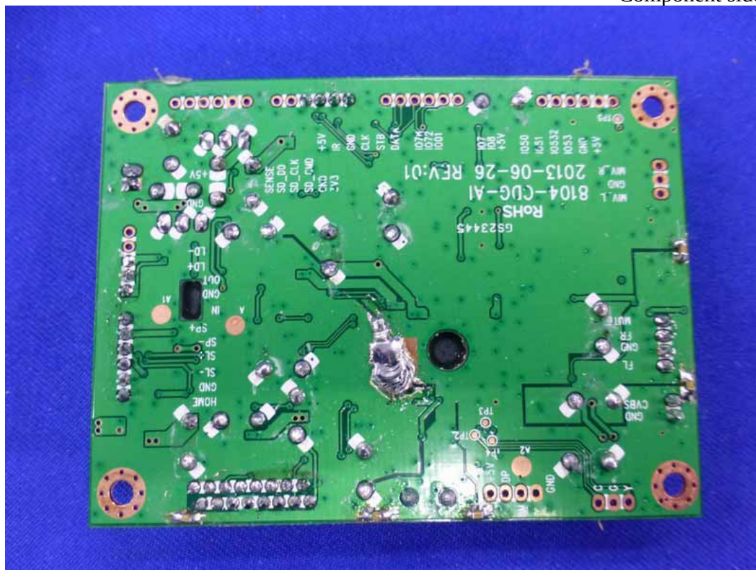
Figure 31 Component side of the PCB
