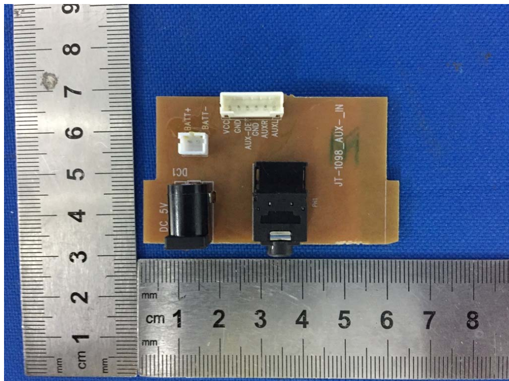
Fig. 14 Component side view of DC jack board
