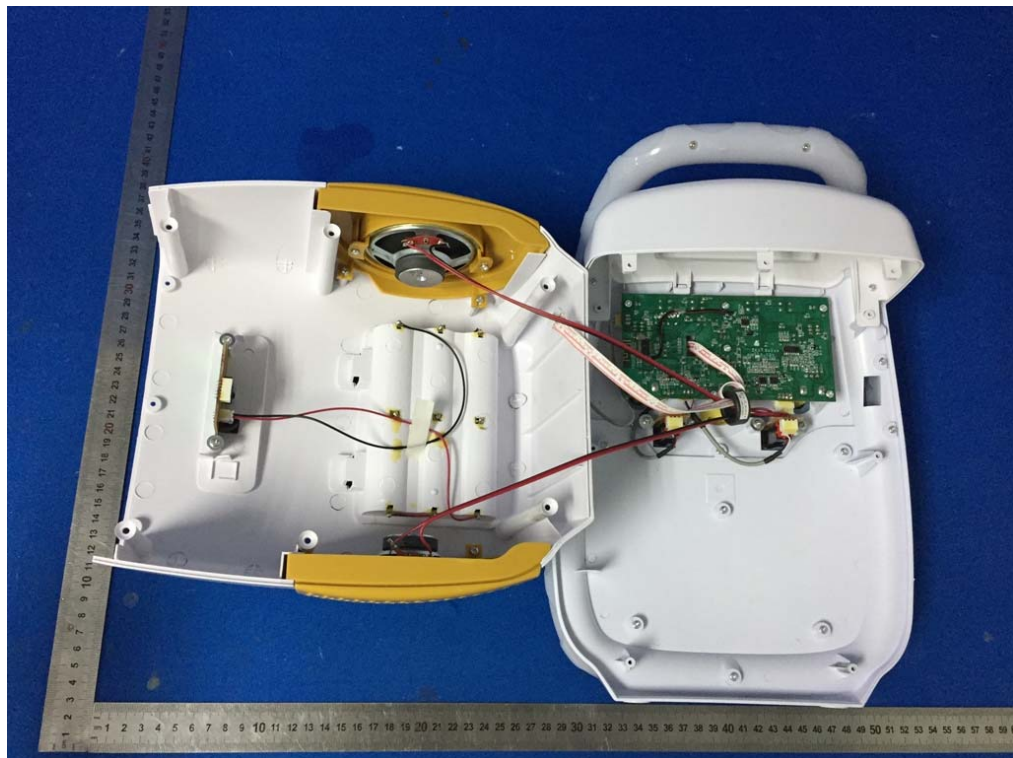
Fig. 10 Internal view of main unit
