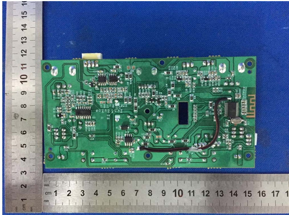
Fig. 15 Trace side view of main board
