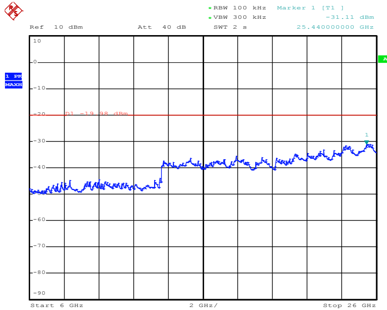
Figure 23: Conducted Spurious Emission, 6 – 26GHz, Mode C
