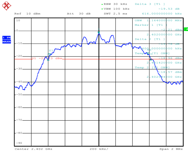
Figure 4: 20dB &99% Bandwidth, Mode A (2402MHz 8DPSK and GFSK)
