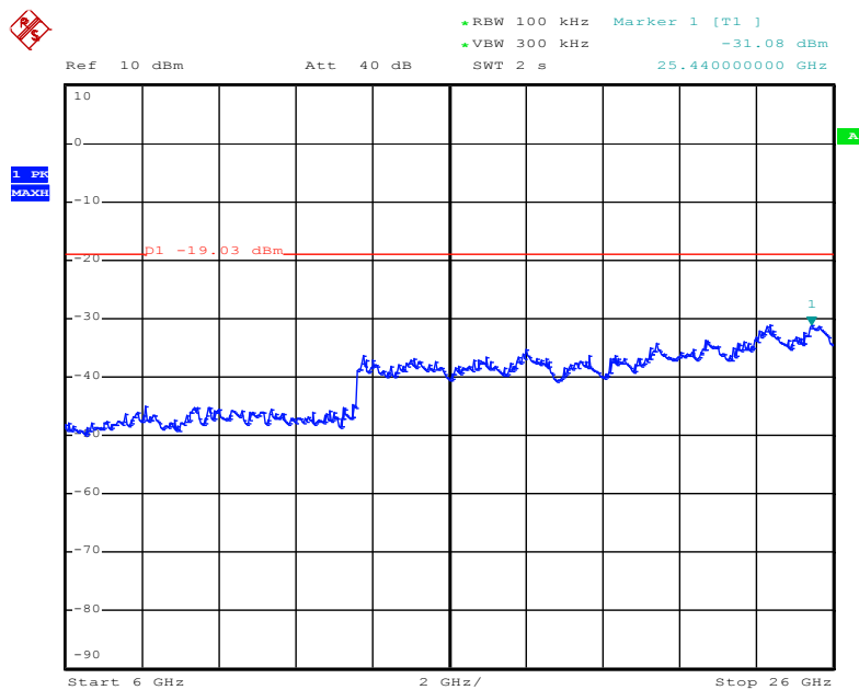
Figure 21: Conducted Spurious Emission, 6 – 26GHz, Mode B
