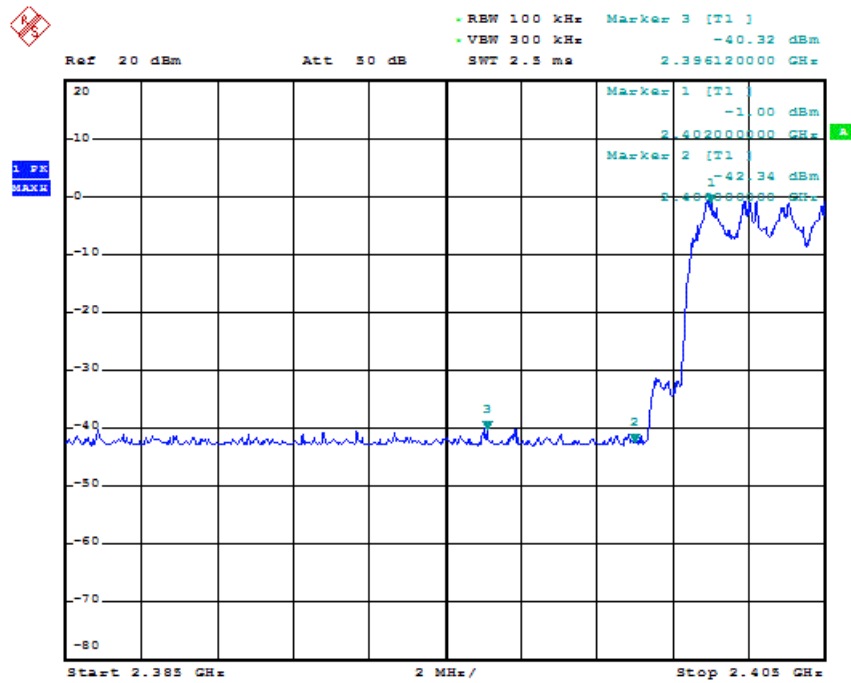
Figure 32: Lower Band Edge Conducted Mode A(Hopping)
