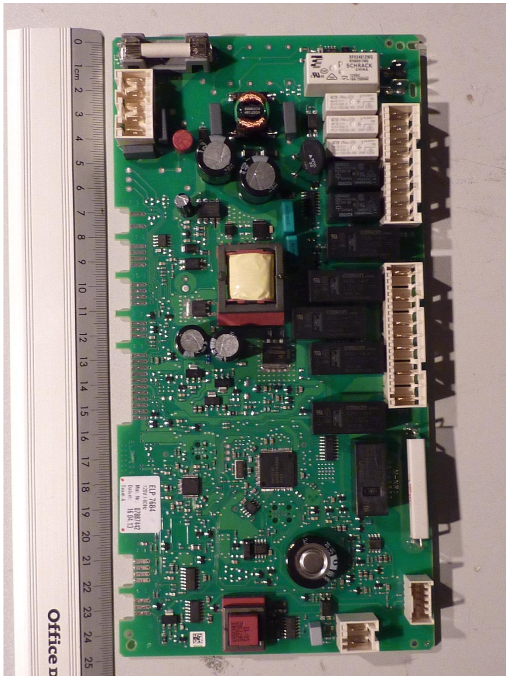
144218_18.JPG: H6700BM, PCB 1, top view
