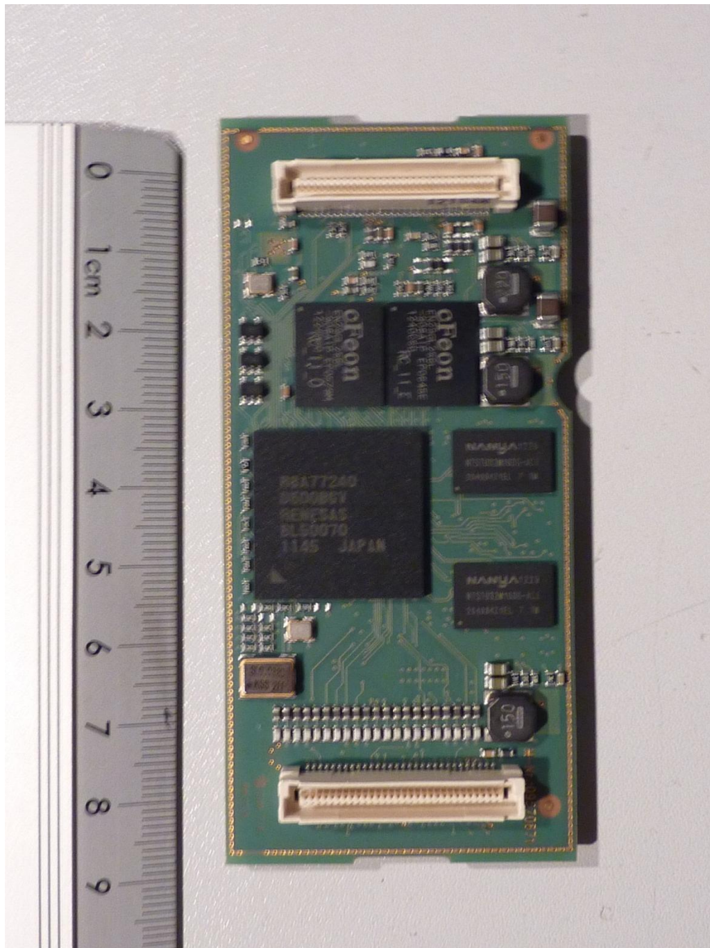
144218_15.JPG: H6700BM, PCB 3, top view
