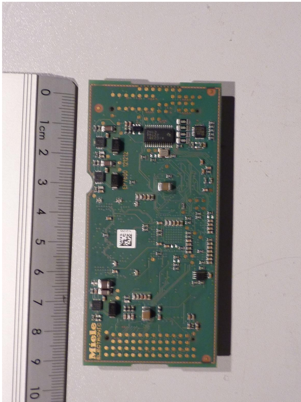
144218_14.JPG: H6700BM, PCB 3, bottom view
