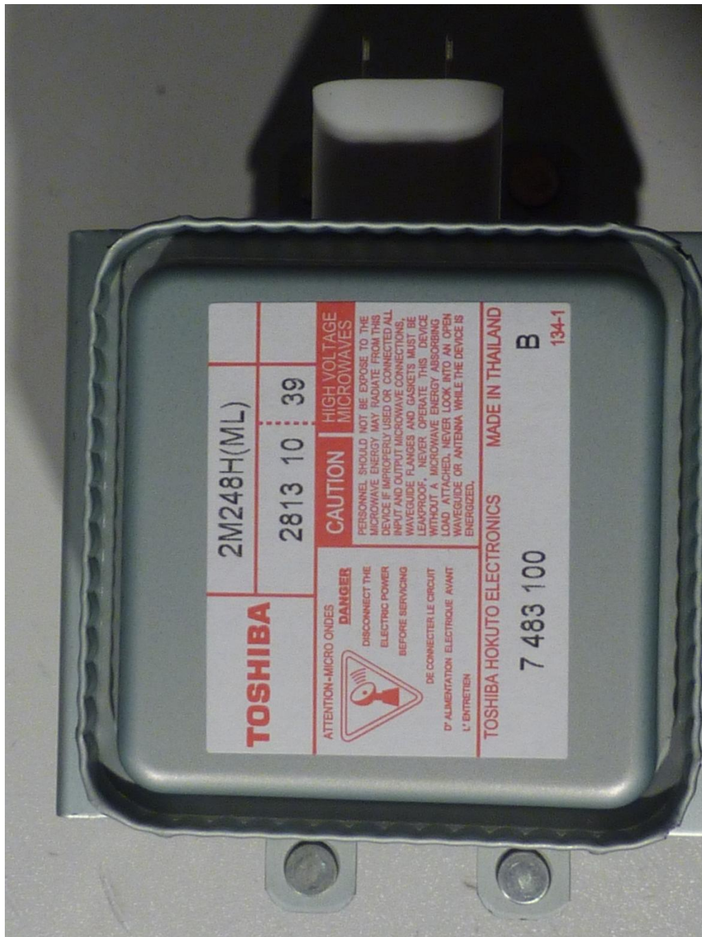
144218_22.JPG: H6700BM, magnetron, type plate
