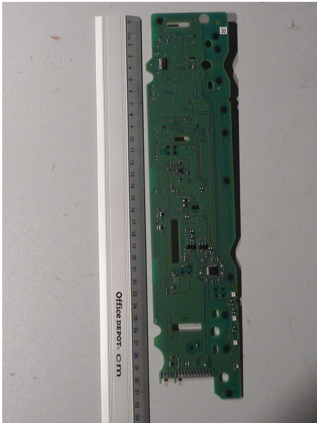
144218_17.JPG: H6700BM, PCB 2, bottom view
