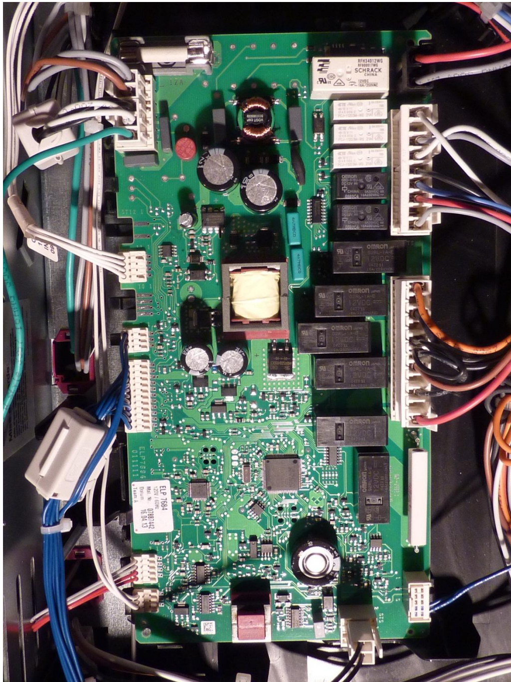
144218_12.JPG: H6700BM, internal view to PBC 1
