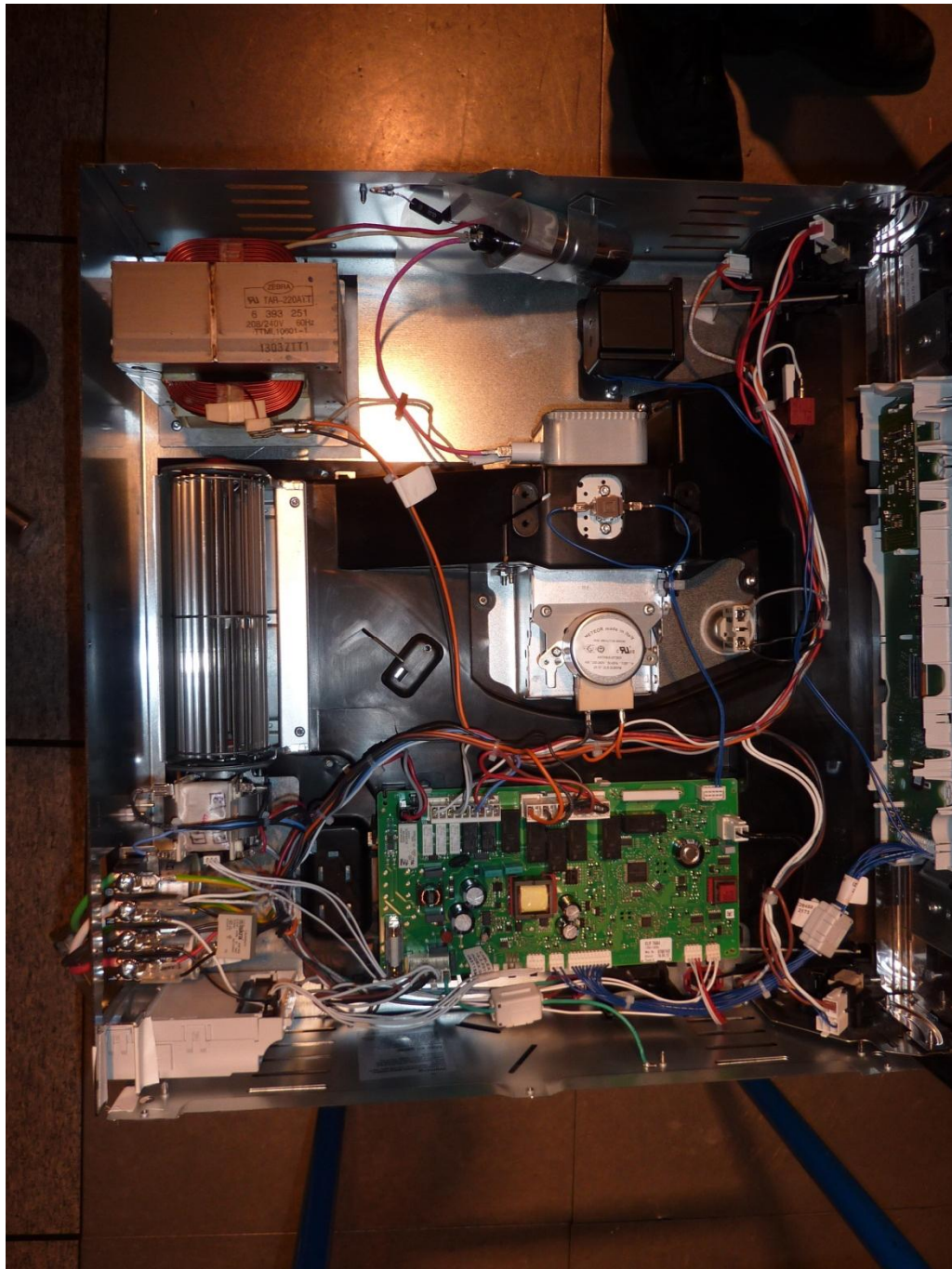
144218_10.JPG: H6700BM, internal view
