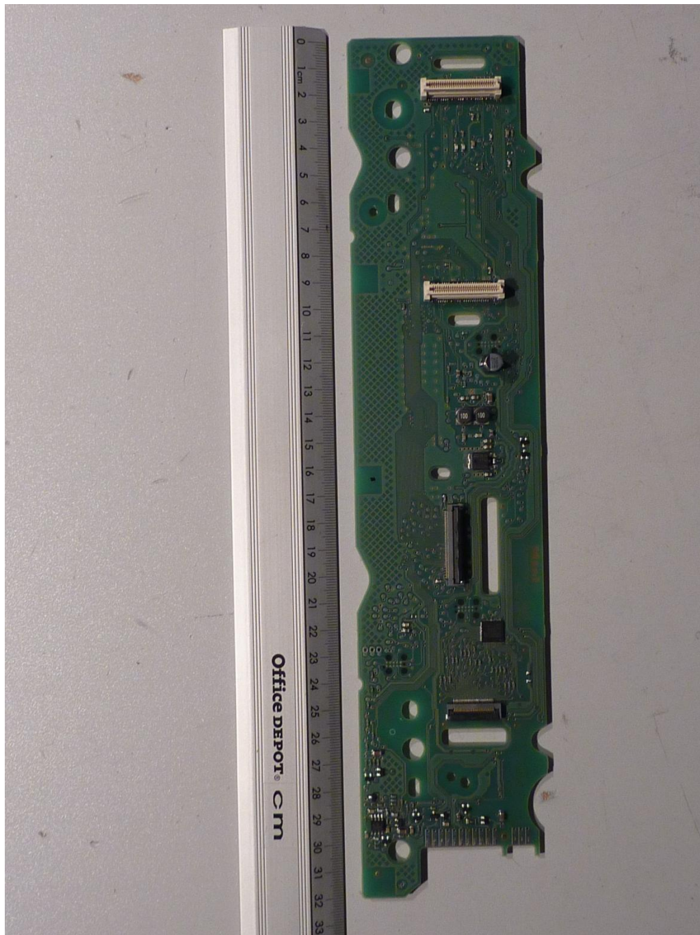
144218_16.JPG: H6700BM, PCB 2, top view
