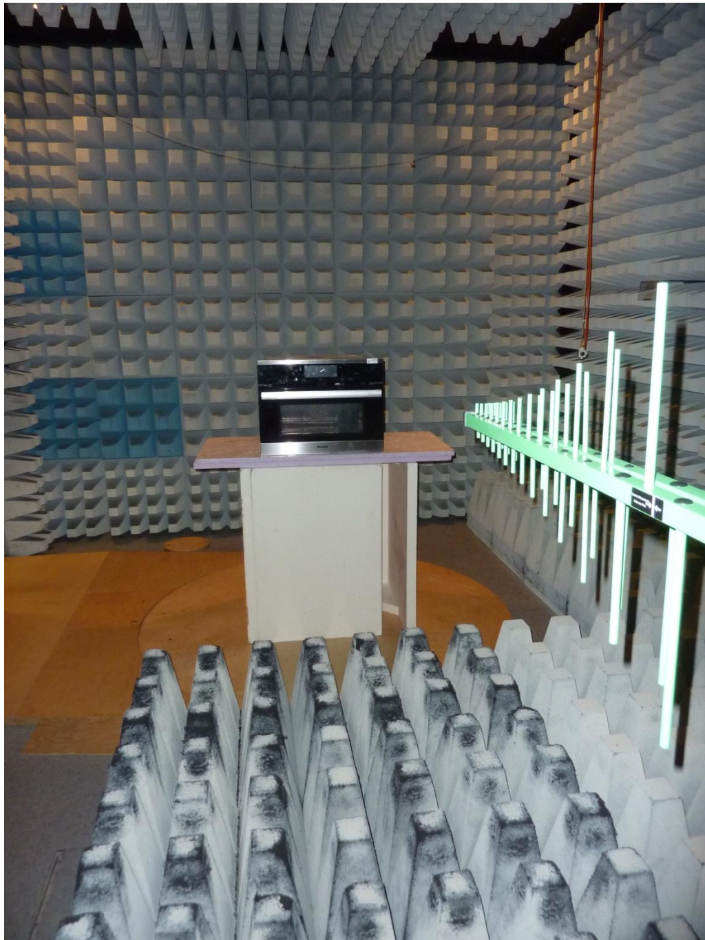
144218_f.JPG: H6700BM, test set-up fully anechoic chamber
