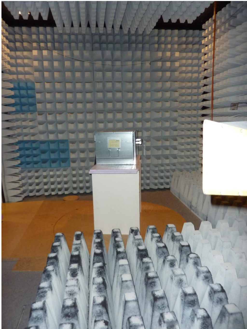
144218_e.JPG: H6700BM, test set-up fully anechoic chamber
